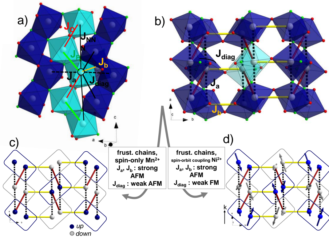
Figure 2: \text{M}_2(\text{SeO}_3)\text{F}_2 crystal structure and labels of the main magnetic exchanges. a,b) inter-chain connections for two projections in the (a,c) and (a,b) planes. O and F are in red and green respectively. The pale blue units allow to distinguish an edge-sharing chain from its (dark blue) neighbors. c-d) projected magnetic structure for c) \text{M} = \text{Mn} , d) \text{M} = \text{Ni} where the rectangles show the projected edge-sharing chains.
