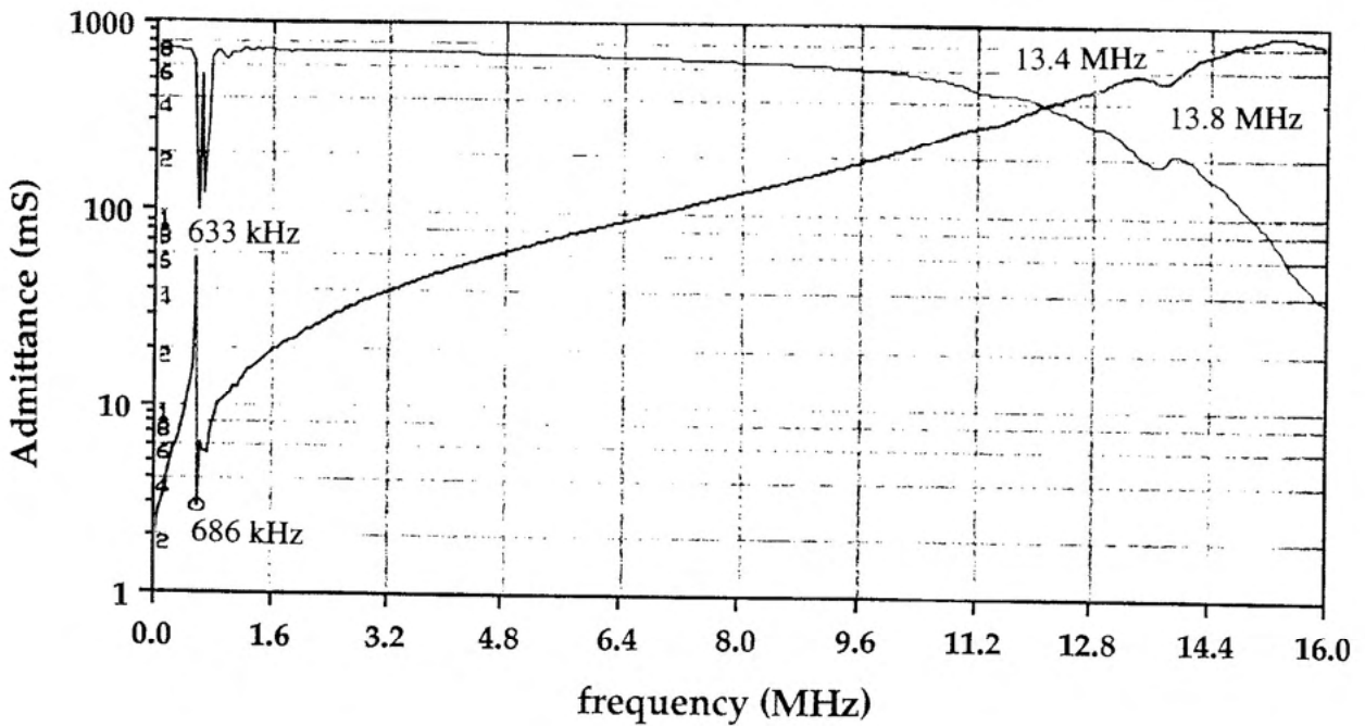
Fig. 22. Admittance spectra of a radially poled PZT hollow sphere transducer: (a) calculated, (b) observed.
