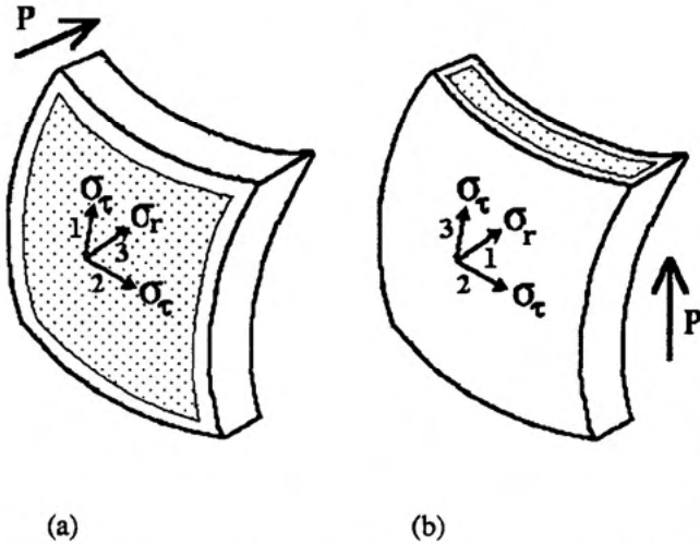
Fig. 8. Transformation of an applied hydrostatic pressure into radial and tangential stresses: (a) radial poling case, (b) top-to-bottom poling case.
