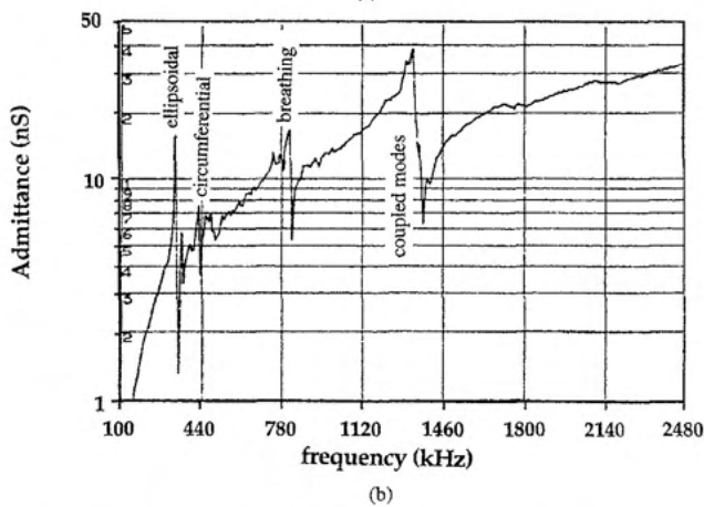
Fig. 4. Admittance spectra of a top-to-bottom poled PZT hollow sphere transducer: (a) calculated, (b) observed.
