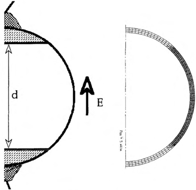
Fig. 3. Polarized region of a top-to-bottom poled sphere.
