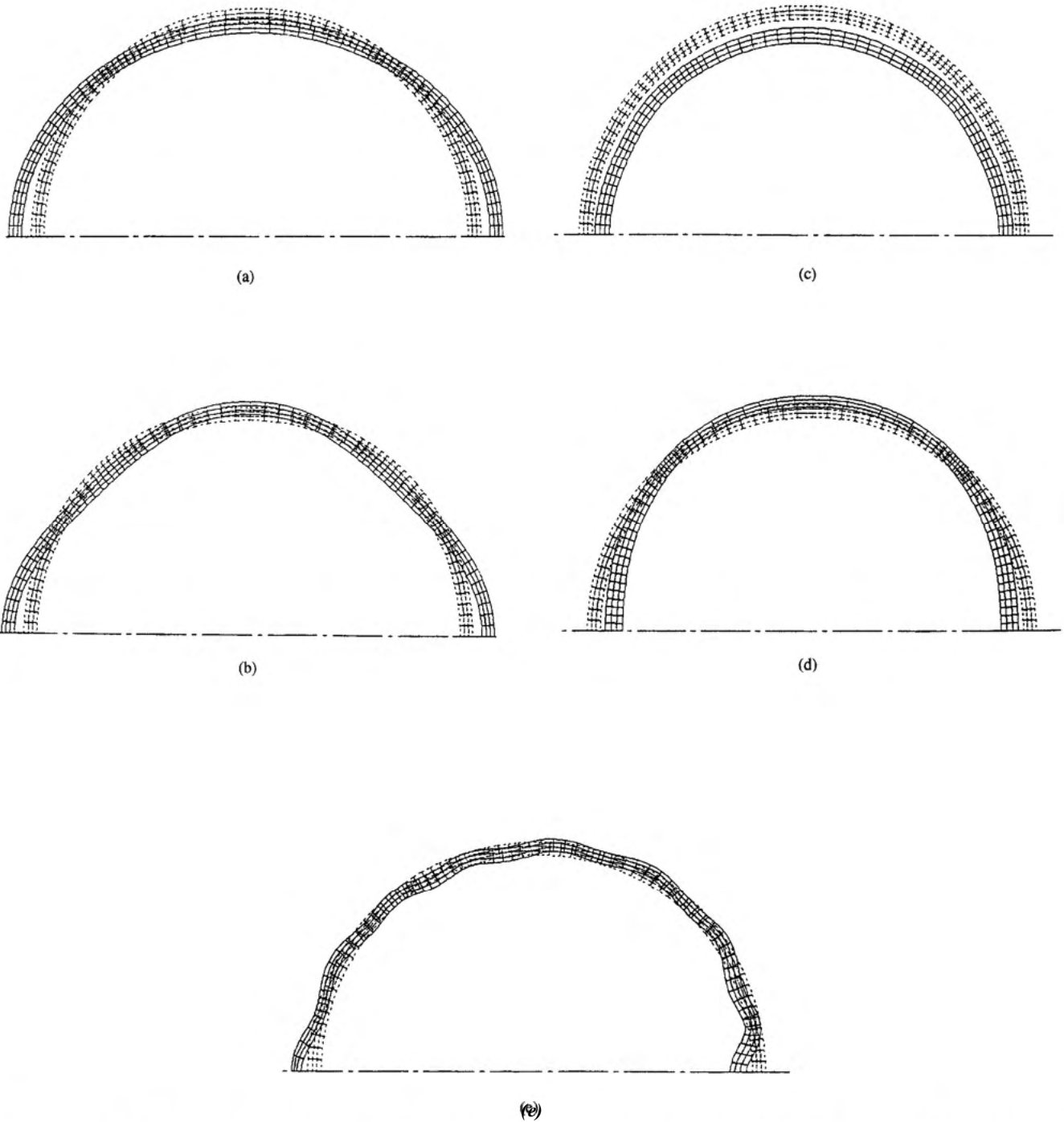
Fig. 5. Modes of vibration of a top-bottom pole piezoelectric hollow sphere: (a) ellipsoidal mode ( f_r \sim 240 kHz); (b) higher order circumferential mode ( f_r = 300 - 400 kHz); (c) breathing mode ( f_r \sim 600 kHz); (d) ellipsoidal + thickness coupled mode ( f_r \sim 1.0 MHz); (e) higher order circumferential + thickness coupled mode ( f_r > 1.0 MHz).
