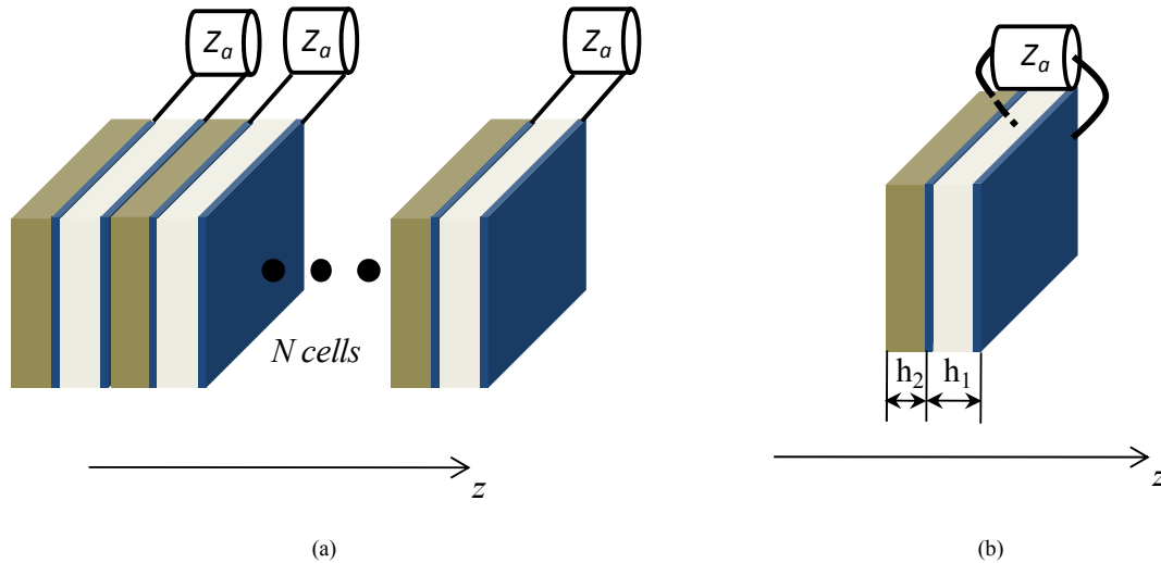
Figure 1: (a) PC composed of passives and active plates, an electrical impedance Z_a is connected to the electrodes of the piezoelectric plates. (b) Unit cell of the PC.
