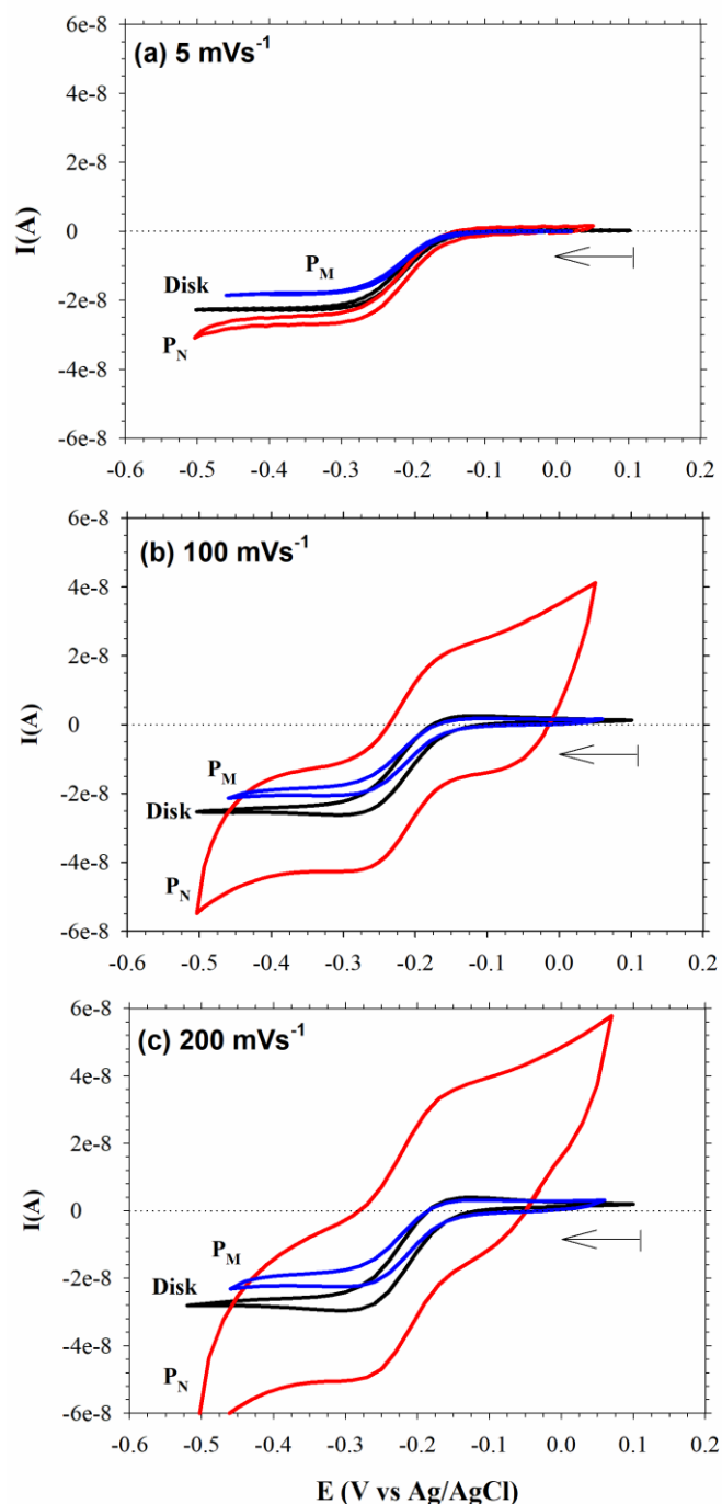
Figure 2. CV responses obtained with the CME filled with P_M and P_N and with a Pt microdisk of the same diameter ( 25 \mu\text{m} ), at three different sweep rates. The initial starting potential and sweep direction are indicated by an arrow. The electrolyte is an aqueous solution of 9 \text{ mmol L}^{-1} [\text{Ru}(\text{NH}_3)_6]\text{Cl}_3 and 0.5 \text{ mol L}^{-1} \text{K}_2\text{SO}_4 , kept under Ar atmosphere.
