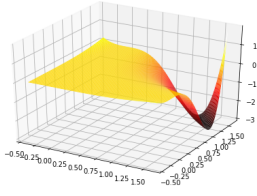
Figure 1: Example of a landscape with a plateau (non-strict saddle point) and a global minimizer.
