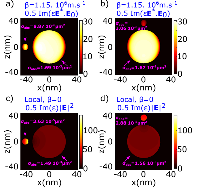
Figure 4. Absorption volume density \alpha_{\text{abs}}(\mathbf{r}) maps for a 5-nm radius nanosphere located in the vicinity of a 25-nm radius nanosphere. The gap between the two spheres is of 5 nm. The HDM parameters for the nanospheres permittivity are the same as Fig.2 and they are also embedded in a background of refractive index n=1.5 . The wavelength is of \lambda=3.1\mu\text{m} (resonance wavelength of the largest sphere). a) and b) \alpha_{\text{abs}}(\mathbf{r}) follows formula (17) with \beta=1.15 \cdot 10^6 \text{m.s}^{-1} ; c) and d) classical Maxwell formula in the local case, i.e. \beta=0 . The absorption volume density is normalized by the norm of the Poynting vector of the incident plane wave. The total heating efficiency \sigma_{\text{abs}} of each particles is indicated in magenta. The sphere is illuminated by a plane wave polarized along the x -axis and propagating at normal incidence along the z axis.
