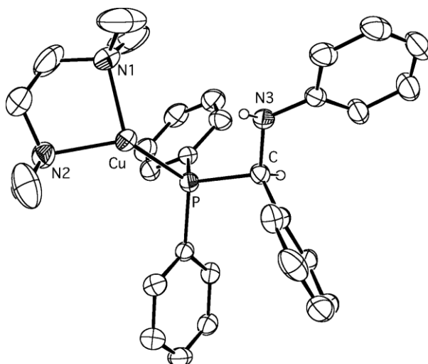
Fig. 1. An ORTEP view of the cation of compound 4. Selected bond distances (Å) and angles (°): Cu-N1, 2.073(6); Cu-N2, 2.104(6); Cu-P, 2.153(2); P-C, 1.878(6); C-N3, 1.466(8); N1-Cu-N2, 87.7(2); N1-Cu-P, 133.9(2); N2-Cu-P, 126.8(2); N3-C-P, 104.8(4).
