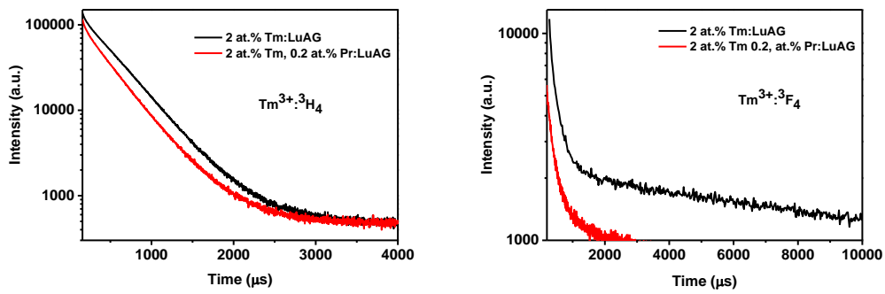
Fig.4. Fluorescence decay curves of the {}^3\text{H}_4 and {}^3\text{F}_4 manifold of Tm:LuAG and Tm,Pr:LuAG crystals.
