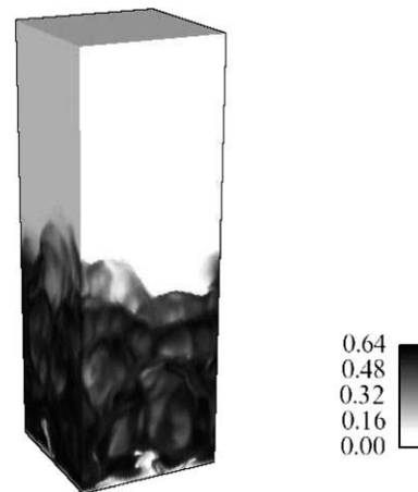
Figure 23. Snapshot of the particle volume fraction in the three-dimensional fluidized bed.
