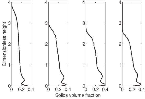
Figure 3. Vertical time-averaged profiles of the particle volume fraction, for x = 1.5 cm.
