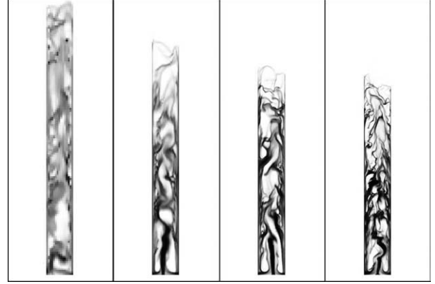
Figure 2. Instantaneous particle volume fraction field in the fluidized bed for different grid mesh sizes.
