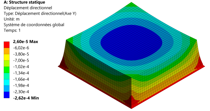
Figure 8: Reference Finite Element simulation: Cooling of a parallelepipedic PDMS block, stuck to a rigid surface at its bottom boundary, from 80 °C down to 20 °C. The color code indicates vertical displacement, in m, from red (zero displacement at the reference bottom boundary) to blue (maximum downward/negative displacement).
