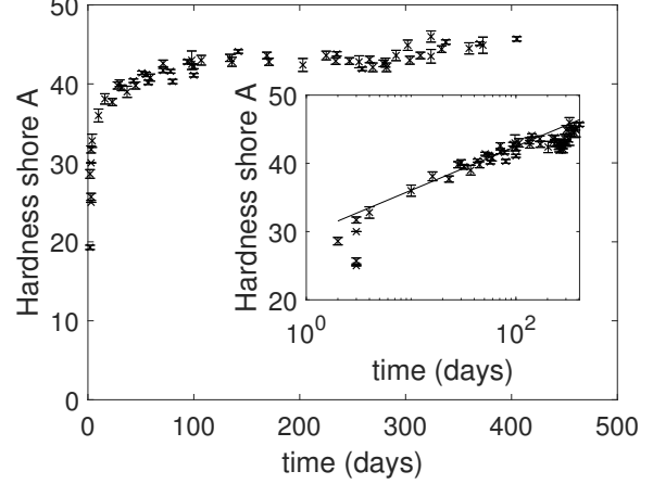
Figure 5: Evolution of the hardness as a function of cross-linking time at 25 ^{\circ}\text{C} . The data include different samples made using different batches. Inset: same data in semi-logarithmic scales. Line: guide for the eye indicating a logarithmic trend.
