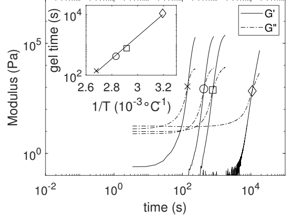
Figure 7: Main: Evolution of the viscoelastic moduli, G' and G'' , as a function of the cross-linking time, for various curing temperatures (40, 70, 80 and 100°C, for the curves from right to left), in log-log scales. Inset: estimated gel time as a function of the inverse of the curing temperature, in semi-log scales. Line: exponential fit.
