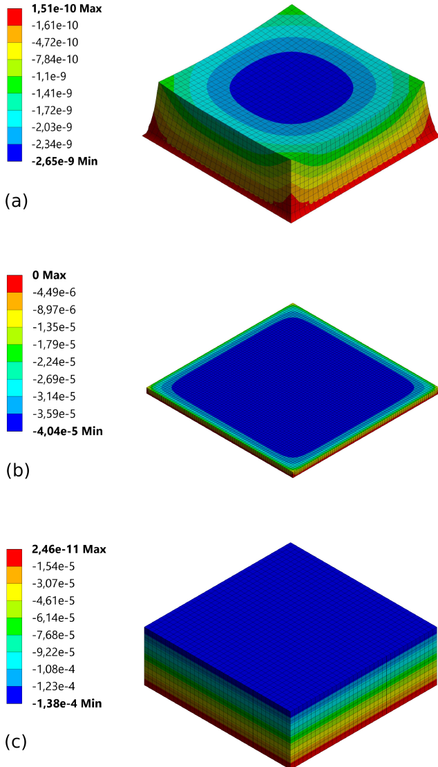
Figure 8: Additional finite element simulations, represented in the same way as in Fig. 7. (a) Same as reference simulation of Fig. 7, but for a sample with all dimensions and mesh size divided by a factor of 10^5 . (b) Same as reference simulation, but for a sample with a thickness divided by a factor of 10. The volume is meshed with rectangular cuboid elements of characteristic size 300\ \mu\text{m} . (c) Same volume and mesh as reference simulation, but when all faces are stress-free.
