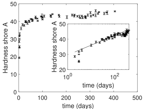
Figure 5: Evolution of the hardness as a function of cross-linking time at 25^\circ\text{C} . Each symbol (error bar) is the mean value (standard deviation) over the five measurements performed on the same sample (see Sec. 2.3). The data include different samples made using different batches. Inset: same data in semi-logarithmic scales. Line: guide for the eye indicating a logarithmic trend.
