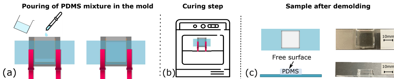
Figure 2: PDMS sample preparation. (a) The aluminum mold (grey part, same as in Fig. 1) is closed by a stack of three glass plates, and the liquid PDMS mixture is poured from top. After curing (b), the sample is carefully demolded, while remaining attached to one of the glass plates (c). The free surface on which profilometry measurements are performed is indicated on the bottom left sketch of (c). Right column of (c): pictures of a typical sample.
