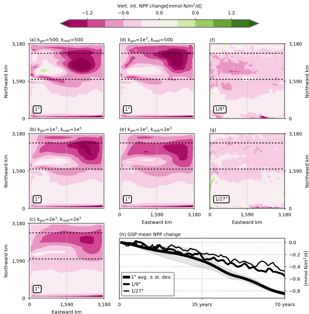
Figure 3. Projected decrease in Net Primary Production (NPP, \text{mmol.N.m}^{-2}.\text{d}^{-1} ) under a high-emission scenario in (a, b, c, d, e) five 1°, (f) 1/9° and (g) 1/27° model simulations. The NPP change is vertically integrated over the entire water column and taken as the difference between the last five years of the climate change and preindustrial control simulations (years 66 to 70). The black dashed horizontal lines delineate the model's subpolar box over which diagnostics for panel (h) and Figures 4, 5, 6 and 7 are performed. This is where simulated NPP is strongest (Fig. 2) and where the simulated NPP decline is also strongest. (h) Time evolution of the NPP decrease in the model's subpolar box in response to climate change, for the three model resolutions. The decrease is computed relative to the preindustrial control simulations. The 1° resolution time series shows the average of the five 1° configurations. Shading indicates \pm one inter-model standard deviation. See Figure A1 over individual model simulations.
