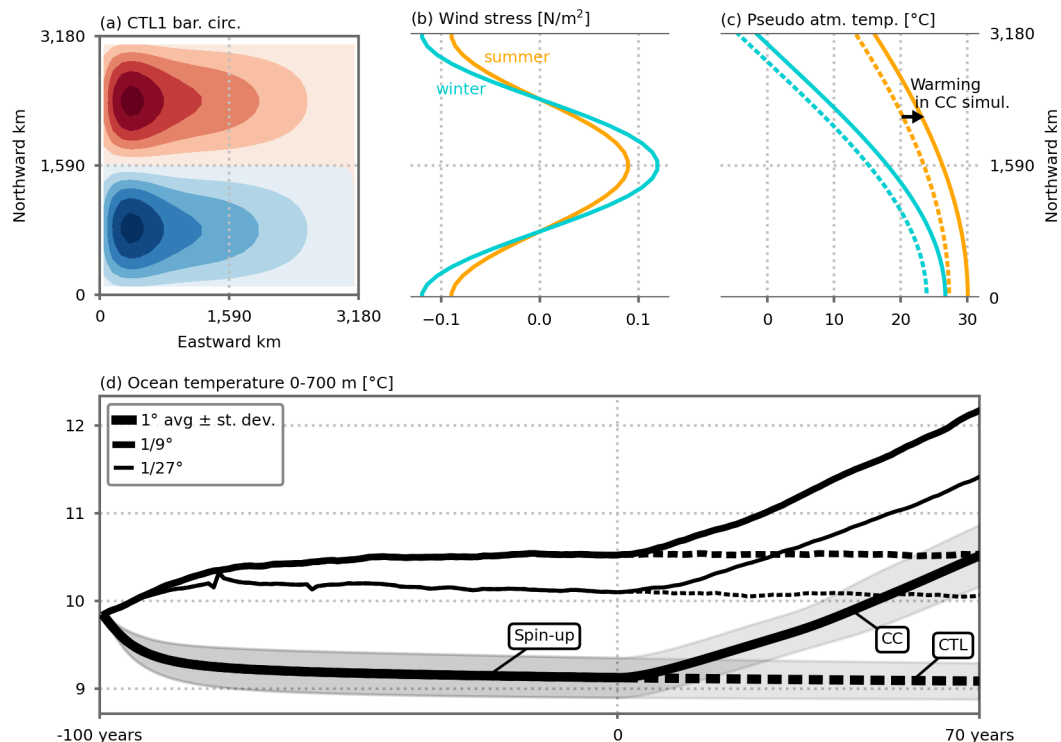
Figure 1. (a) Barotropic circulation over the model domain (average of the five 1^{\circ} resolution preindustrial control simulations, see also Fig. A2 for individual configurations) and analytical external forcings as a function of latitude: (b) wind stress ( N \cdot m^{-2} ), and (c) pseudo atmospheric temperature ( ^{\circ}C ). The forcings vary seasonally in a sinusoidal manner between winter (blue) and summer (orange) extrema. In the climate change simulations, the pseudo atmospheric temperature increases linearly in time between the dashed and solid lines (panel c). After 70 years of simulation, the linear atmospheric temperature increase reaches +2.8^{\circ}C . (d) Time series of annual ocean temperature ( ^{\circ}C ) averaged between 0 and 700 metres depth over the model domain. Years -100 to 0 correspond to the spin-up period under seasonal preindustrial forcing. The preindustrial control and climate change simulations discussed in this paper start at year 0. The 1^{\circ} resolution time series shows the average of the five 1^{\circ} configurations. Shading indicates \pm one standard deviation. See Fig. A1 for individual 1^{\circ} model configurations. The small peaks in the time series of the 1/27^{\circ} resolution spin-up around years -80 and -60 are due to a problem during the chaining of the spin-up jobs (which were set by periods of 2 years). These errors did not influence the equilibrium states and we decided not to rerun the spin-up simulations to save computational resources.
