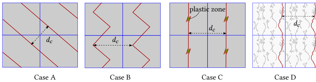
Figure 21: Periodic- crack spacing in micro-structures.
