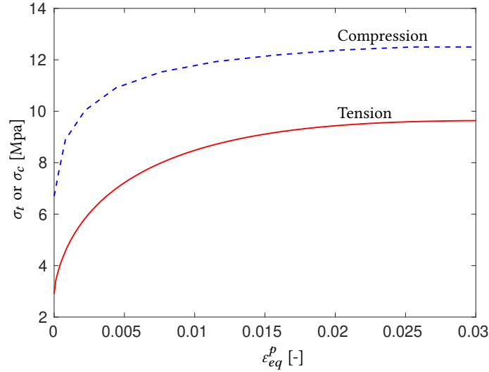
Figure 16: Hardening curves for the plasticity model
