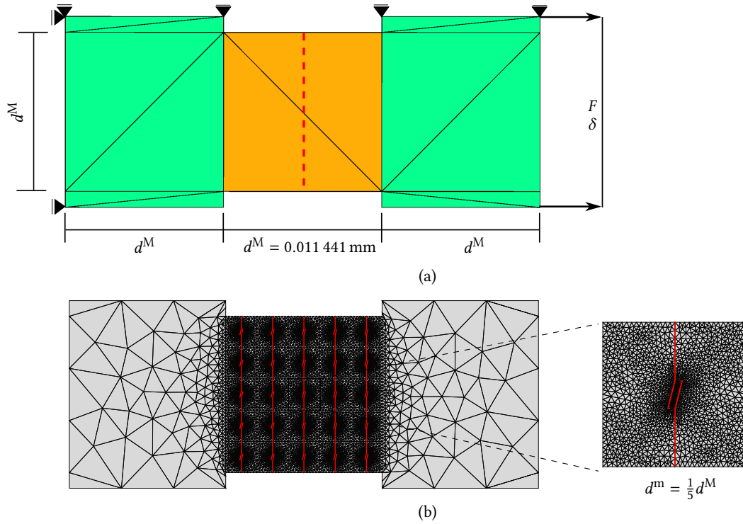
Figure 19: h study- case C. (a) macroscale problem shown in FE discretization; (b) FE mesh for DNS analysis with red lines dictating initial zero-thickness cohesive elements and the adopted micromodel.
