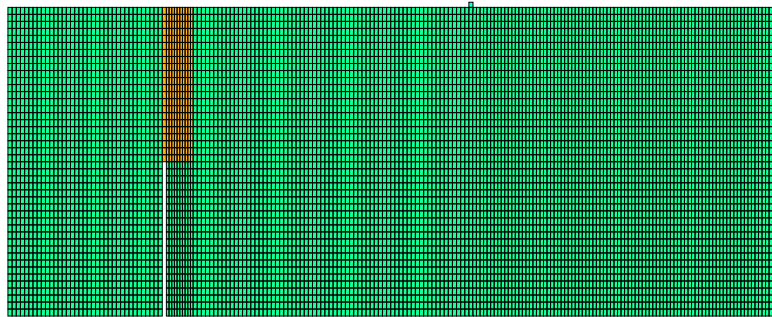
Figure 26: Macroscale mesh for mix-mode failure test
