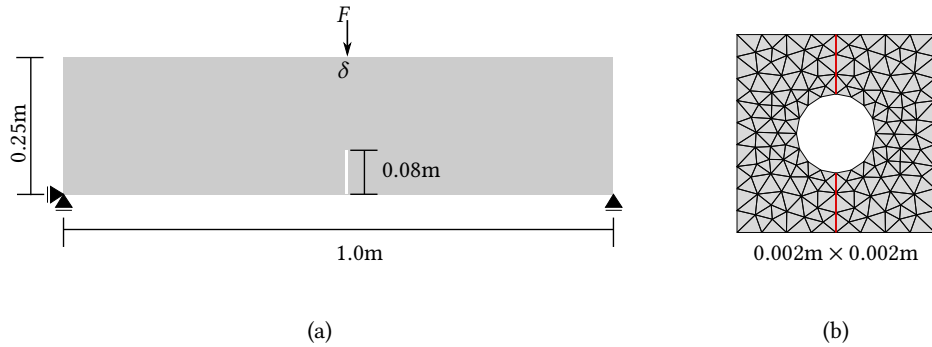
Figure 13: Three point bending test. (a) macroscale problem description; (b) micromodel which is allowed to open at the central vertical line.
