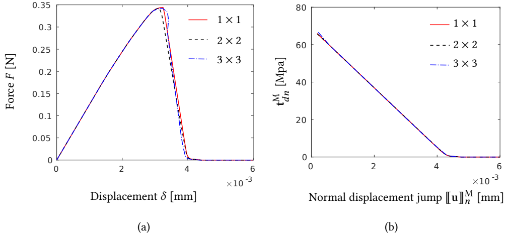
Figure 12: Objective results with respect to the size of the micromodel with complex crack pattern. (a) force-displacement curves; (b) homogenized cohesive laws in normal direction.
