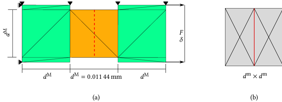
Figure 9: Uniaxial tensile test with pre-defined micro-crack patterns. (a) macroscale problem description (shown in FE discretization); (b) micromodel which is allowed to open at the central vertical line and discretized by six-node triangular elements.
