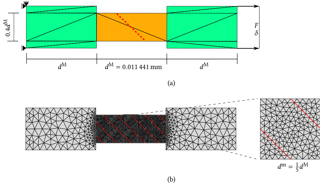
Figure 17: h study- case A. (a) macroscale problem shown in FE discretization; (b) FE mesh for DNS analysis with red lines dictating initial zero-thickness cohesive elements and the adopted micromodel.
