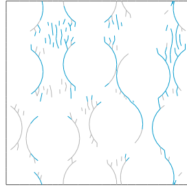
Figure 24: Cohesive cracks in the micromodel at the moment of bifurcation in case D. Blue lines indicate loading cracks while grey lines indicate unloading cracks.
