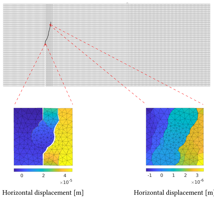
Figure 27: Curved macroscale crack with snapshots of micromodels at time-step indicated by point A in Figure 28
