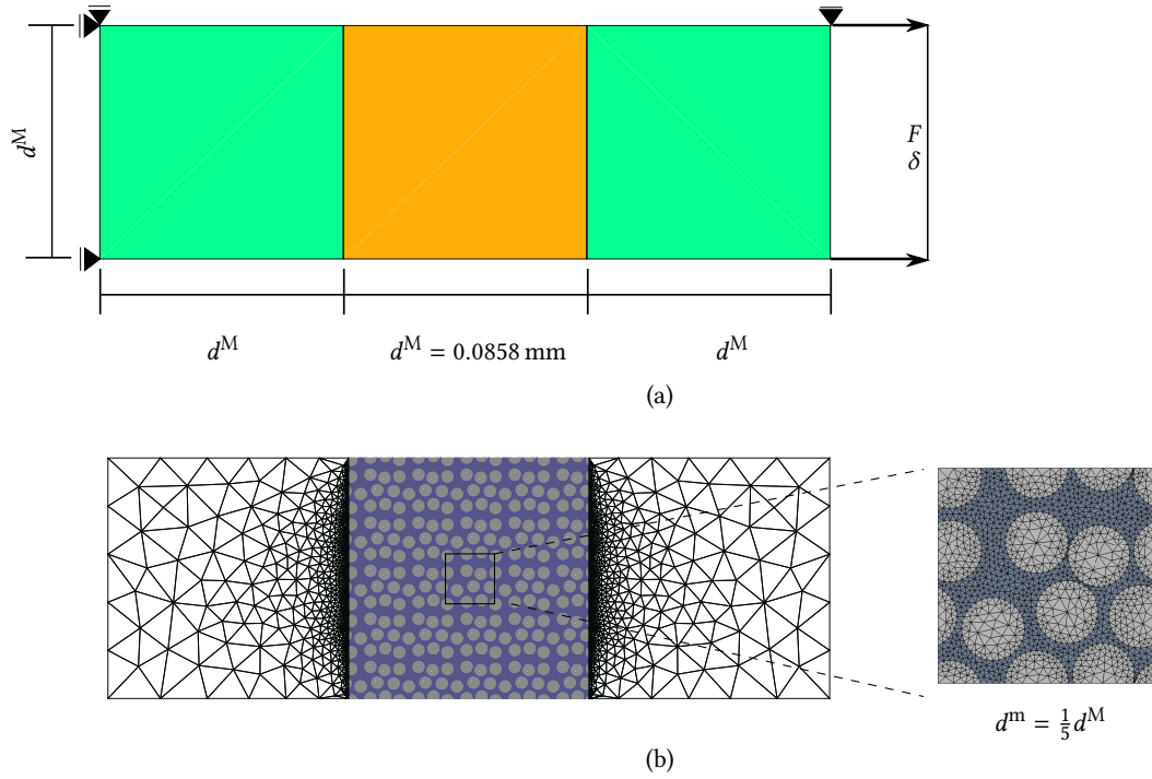
Figure 20: h study- case D. (a) macroscale problem shown in FE discretization; (b) FE mesh for DNS analysis and the adopted micromodel.
