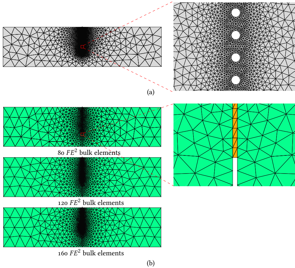
Figure 14: Finite element mesh for three point bending test. (a) DNS analysis mesh; (b) macroscale mesh for two-scale CH analysis with different discretizations along the central band.
