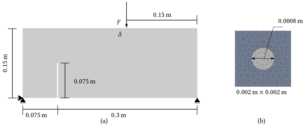
Figure 25: Mix-mode failure test. (a) macroscale problem description; (b) micromodel discretized by six-node triangular elements.
