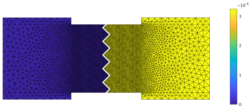
Figure 22: Horizontal displacement (in mm) at the end of simulation of DNS analysis in case B.
