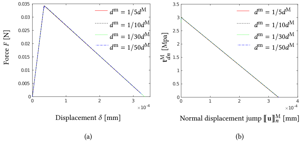
Figure 10: Objective results with respect to the size of the micromodel with regular crack pattern. (a) force-displacement curves; (b) homogenized cohesive laws in normal direction.
