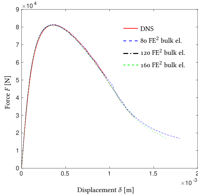
Figure 15: Force-displacement curves of three point bending tests
