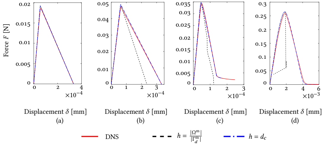
Figure 23: Force-displacement curves of h study tests. (a) case A; (b) case B; (c) case C; (d) case D.
