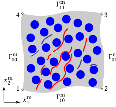
Figure 4: Strong periodic BCs on RVE, which reads \mathbf{u}_{\Gamma_{01}^m} = \mathbf{u}_{\Gamma_{00}^m} + \mathbf{u}_2 - \mathbf{u}_1 and \mathbf{u}_{\Gamma_{11}^m} = \mathbf{u}_{\Gamma_{10}^m} + \mathbf{u}_4 - \mathbf{u}_1 .
