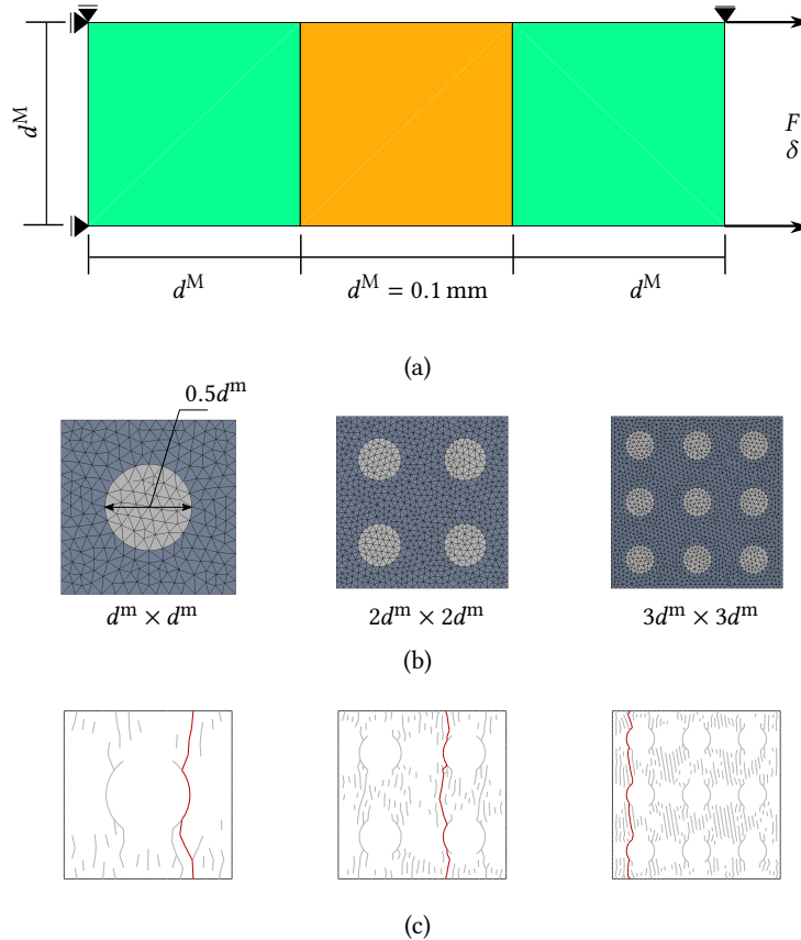
Figure 11: Uniaxial tensile test with complex micro-crack pattern. (a) macroscale problem description (shown in FE discretization); (b) micromodels which are discretized by six-node triangular elements; (c) final micro-failure patterns (red lines indicate completely failed cracks while grey lines indicate unloading cracks).
