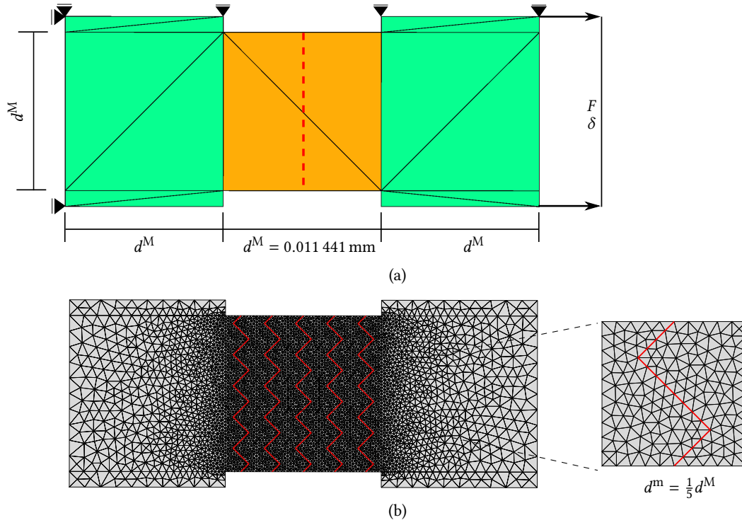
Figure 18: h study- case B. (a) macroscale problem shown in FE discretization; (b) FE mesh for DNS analysis with red lines dictating initial zero-thickness cohesive elements and the adopted micromodel.
