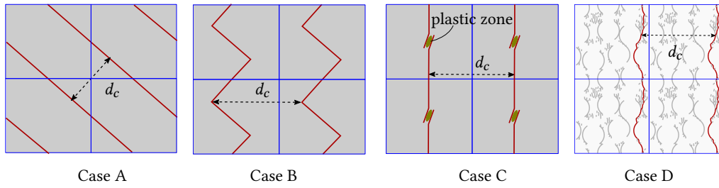
Figure 21: Periodic- crack spacing in micro-structures.
