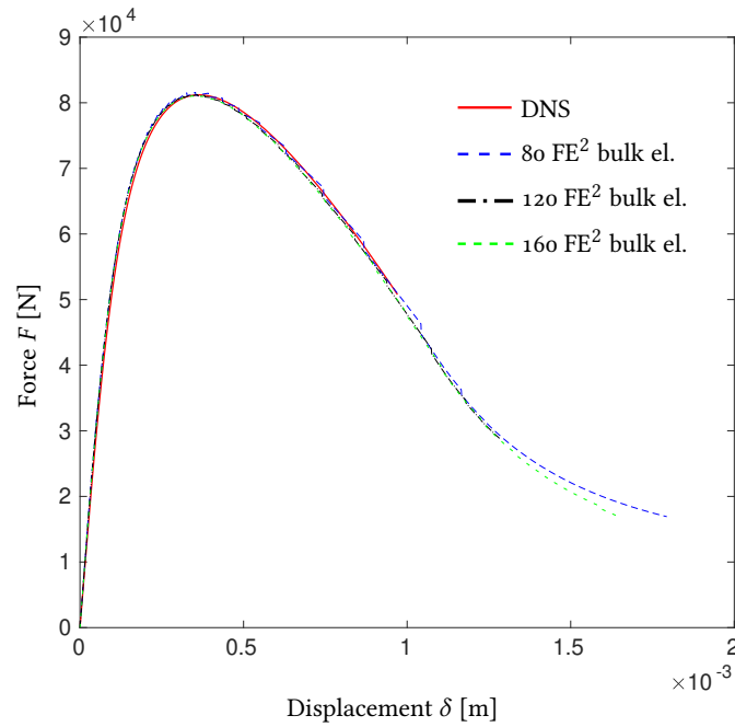
Figure 13: Force-displacement curves of three point bending tests
