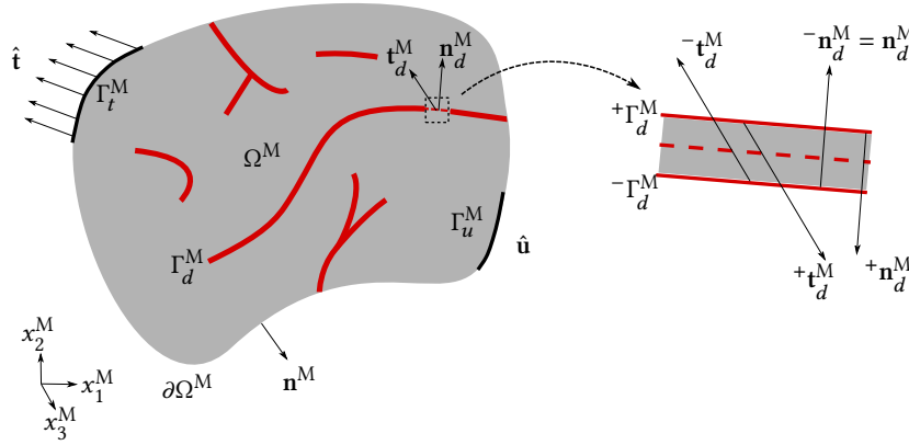
Figure 1: Schematic representation of macroscopic failure problem with cohesive cracks.
