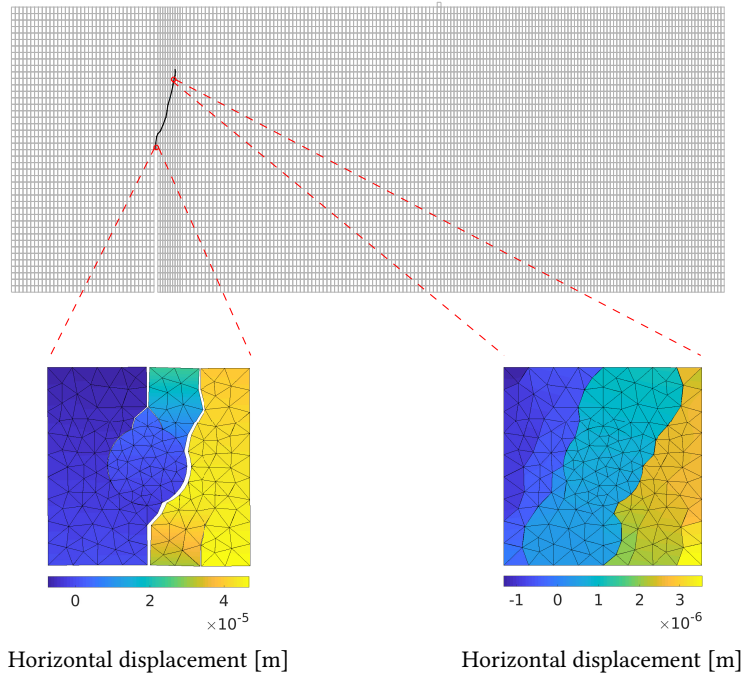
Figure 22: Curved macroscale crack with snapshots of micromodels at time-step indicated by point A in Figure 23
