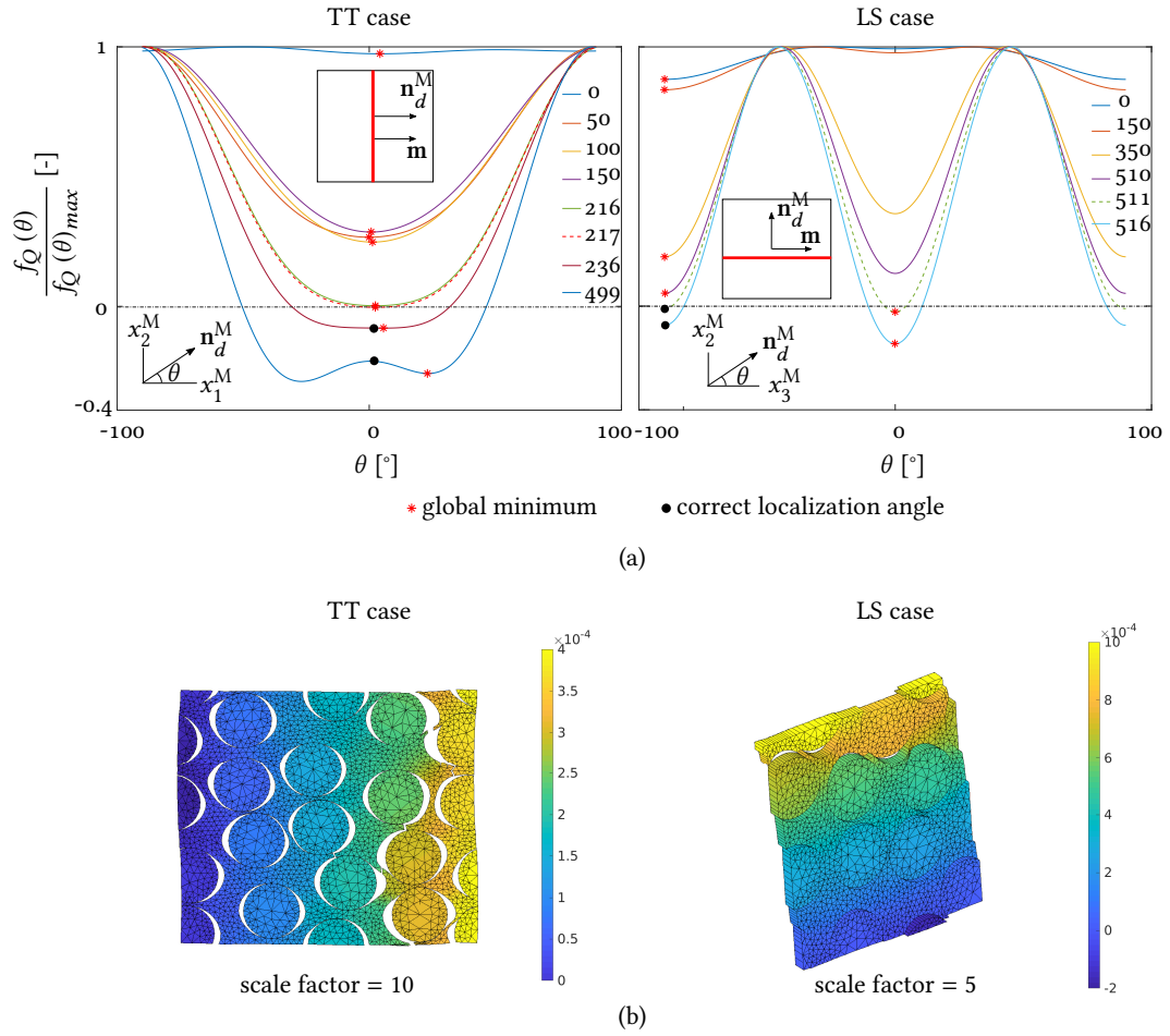
Figure 8: Bifurcation mode analysis. (a) evolution of f_Q(\theta) normalized by its maximum value; (b) deformation of micromodels at time of bifurcation.
