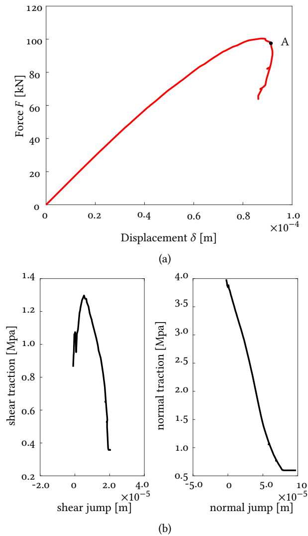
Figure 23: Macroscale response. (a) Force-displacement curve; (b) homogenized traction-separation law of first cohesive point on macro-crack
