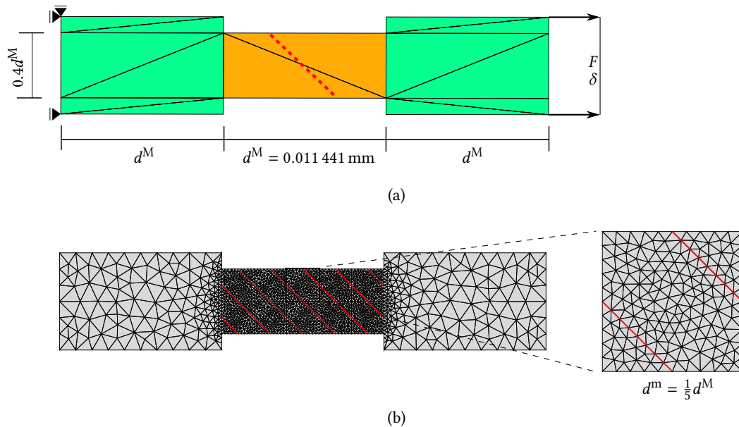
Figure 15: h study- case A. (a) macroscale problem shown in FE discretization; (b) FE mesh for DNS analysis and the adopted micromodel.
