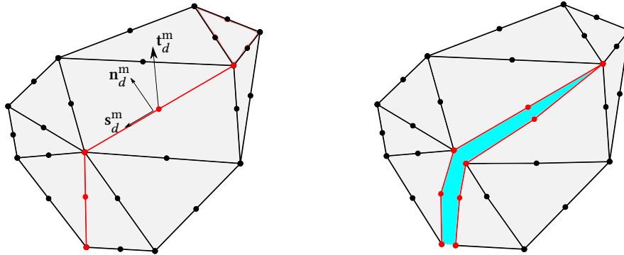
Figure 5: Insertion of cohesive elements during the simulation.
