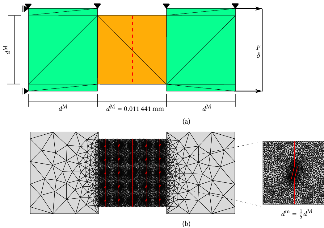
Figure 17: h study- case C. (a) macroscale problem shown in FE discretization; (b) FE mesh for DNS analysis and the adopted micromodel.
