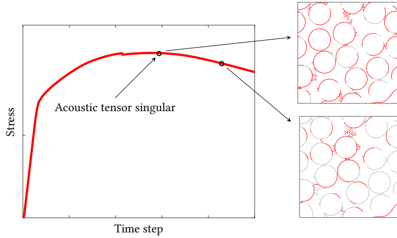
Figure 2: Microscale failure mechanism at different load steps. Red lines in the micromodel show cohesive cracks that are damaging, while gray lines represent unloading cracks.
