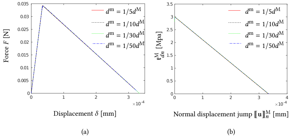
Figure 10: Objectivity with respect to the size of the micromodel. (a) force-displacement curves; (b) homogenized cohesive laws in normal direction.
