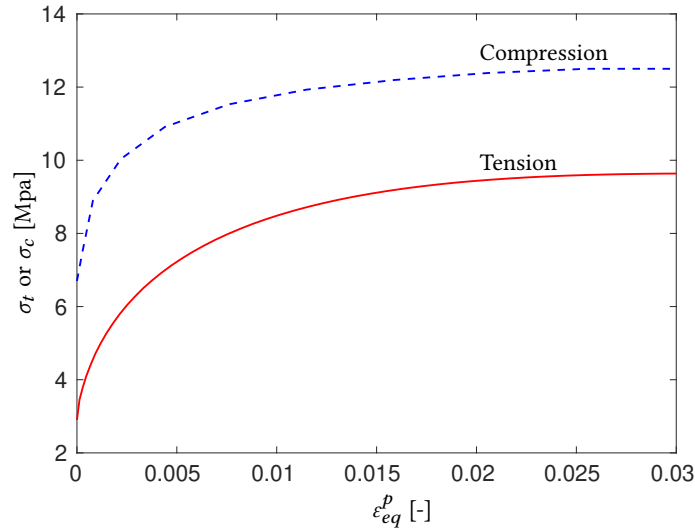
Figure 14: Hardening curves for the plasticity model
