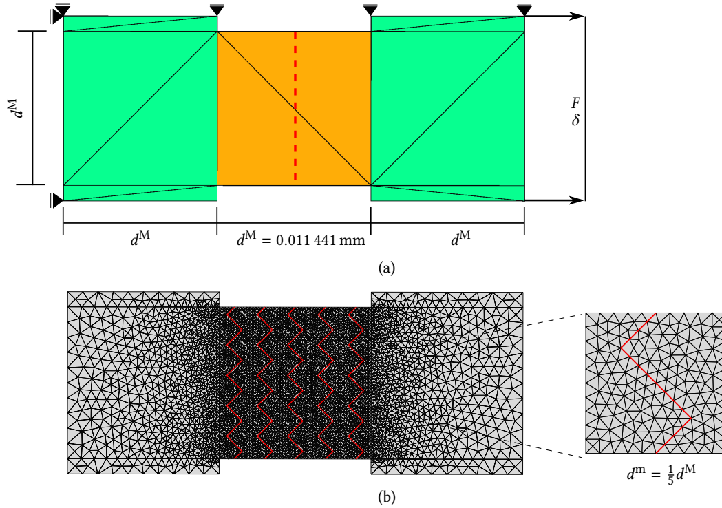
Figure 16: h study- case B. (a) macroscale problem shown in FE discretization; (b) FE mesh for DNS analysis and the adopted micromodel.
