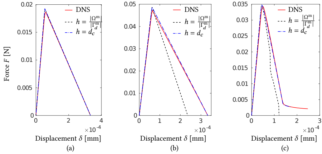
Figure 19: Force-displacement curves of h study tests. (a) case A; (b) case B; (c) case C.
