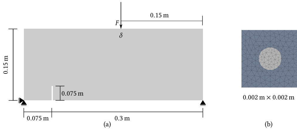
Figure 20: Mix-mode failure test. (a) macroscale problem description; (b) micromodel discretized by six-node triangular elements.
