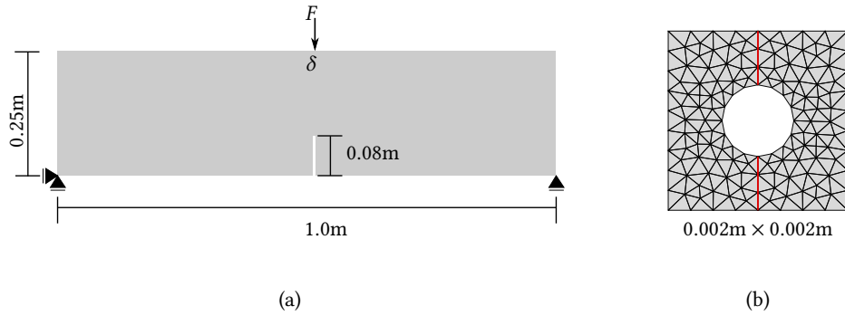
Figure 11: Three point bending test. (a) macroscale problem description; (b) micromodel which is allowed to open at the central vertical line.
