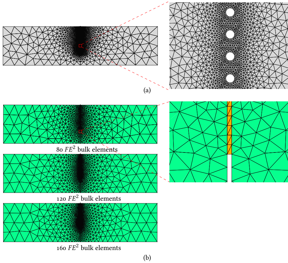
Figure 12: Finite element mesh for three point bending test. (a) DNS analysis mesh; (b) macroscale mesh for two-scale CH analysis with different discretizations along the central band.
