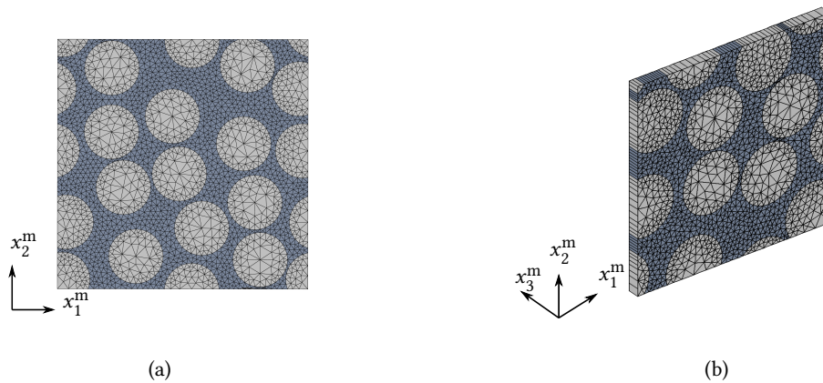
Figure 7: Micromodels used for bifurcation mode analysis. (a) micromodel for TT case; (b) micromodel for LS case.
