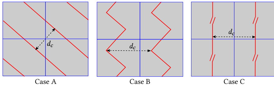
Figure 18: Minimum crack spacing in micro-structures.
