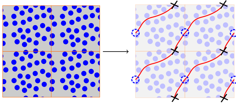
Figure 6: Periodic cracking pattern in pairs of RVE boundary nodes.
