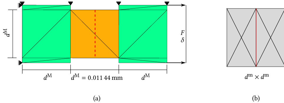
Figure 9: Uniaxial tensile test. (a) macroscale problem description (shown in FE discretization); (b) micromodel which is allowed to open at the central vertical line and discretized by six-node triangular elements.
