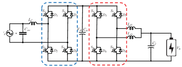
Figure 9: Grid to Vehicle
