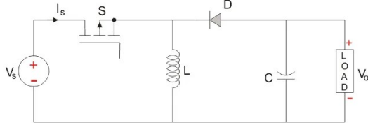
Figure 7: Buck-Boost converter
