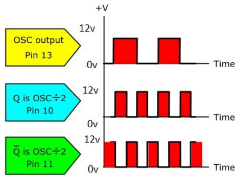
Figure 5: Waveform signal of three output
