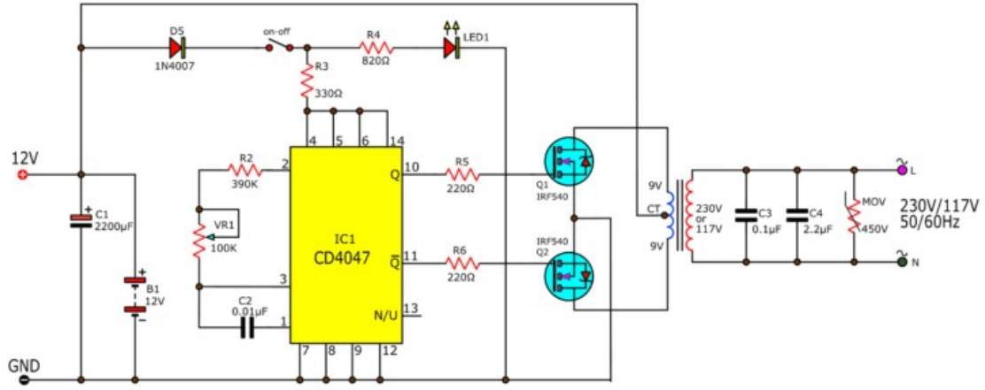
Figure 6: Inverter circuit
