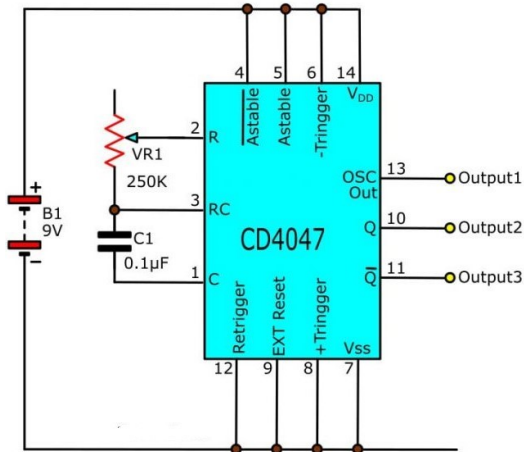
Figure 4: Square wave generator
