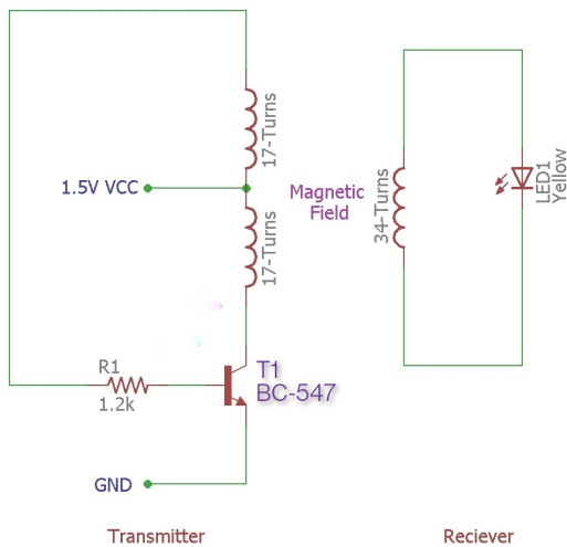
Figure 11: Wireless Power Transfer Circuit
