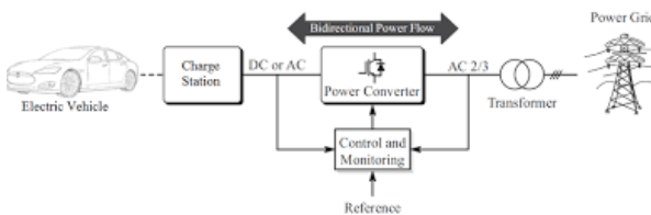
Figure 1: V2G system.
