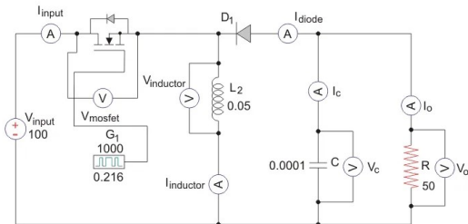
Figure 8: Buck-Boost converter
