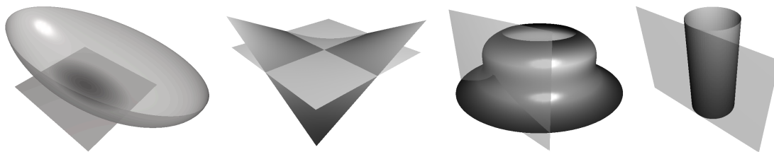
Figure 7.6: Elliptic, left, hyperbolic, center, and parabolic, the two last on the right, points.
