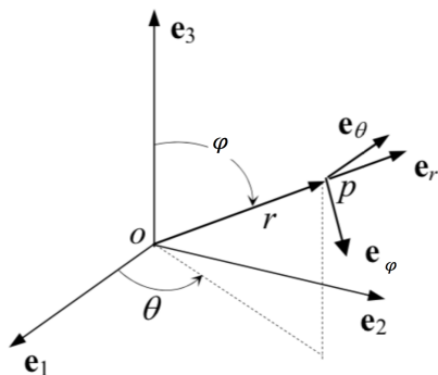
Figure 5.3: Spherical coordinates.
