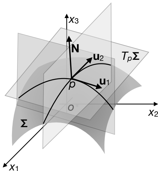
Figure 7.5: Principal curvatures.
