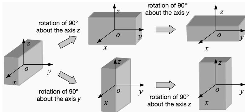
Figure 2.3: Non-commutativity of the rotations.
