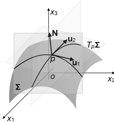
Figure 7.5: Principal curvatures.
