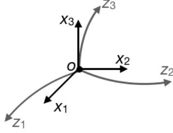
Figure 6.1: Cartesian and curvilinear coordinates.
