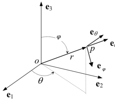
Figure 4.10: Spherical coordinates.
