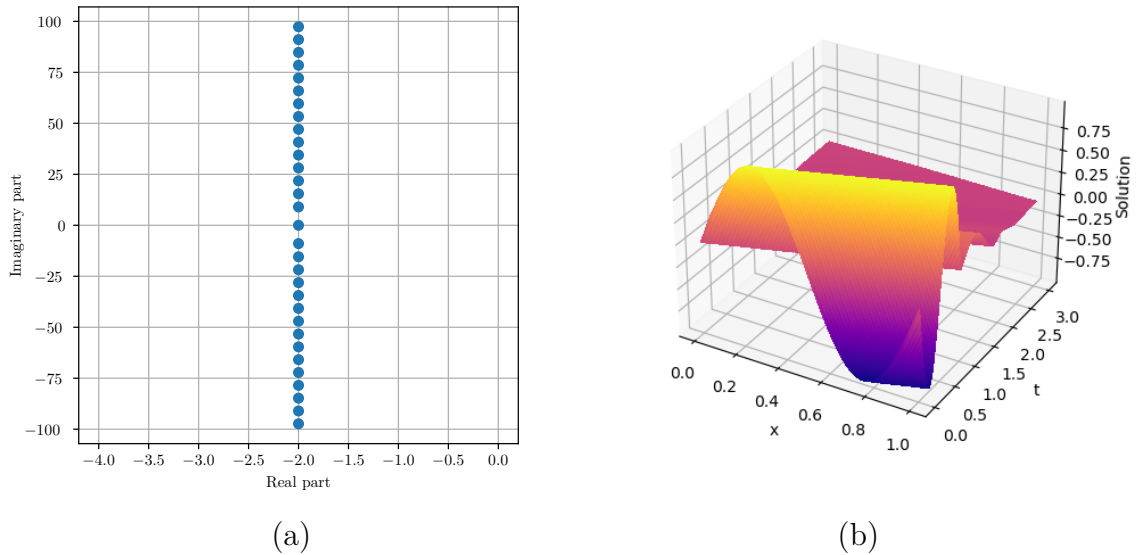
Figure 4.1: (a) Spectrum distribution of (4.8) and (b) solution of (4.6) with initial condition \varphi(0, x) = \sin(2\pi x) , with \frac{L}{\lambda} = 1 and parameters k_p and k_i satisfying (4.9).
