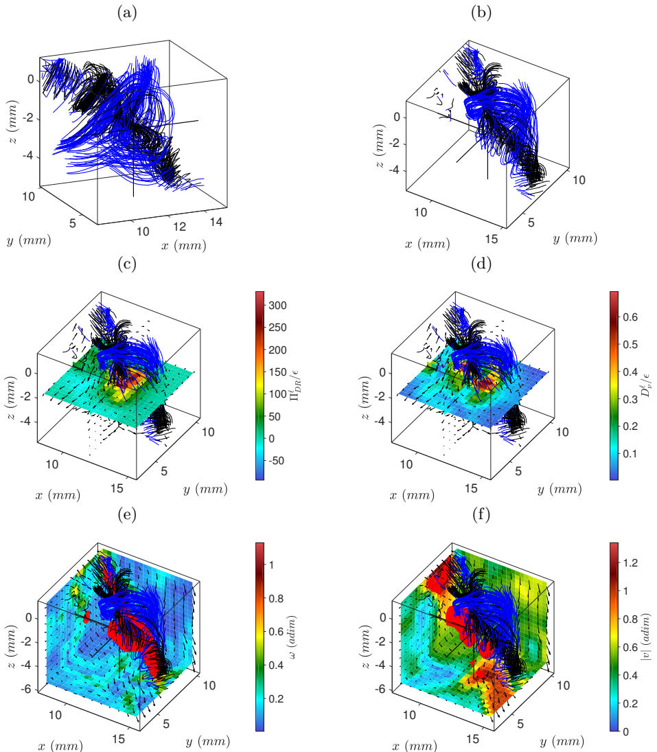
FIGURE 9. Velocity field around the 1 st extreme event of \Pi_{DR}^l of case T1. (a) Velocity streamlines. (b) Velocity streamlines from another point of view. (c) In-plane velocity field (arrows) and \Pi_{DR}^l field (color) in the (xy) plane containing the extreme event. (d) In-plane velocity field (arrows) and \mathcal{D}_v^l field (color) in the (xy) plane containing the extreme event. (e) In-plane velocity field (arrows) in three (xy), (xz) and (yz) planes bounding the observed area, vorticity norm (color on these planes), velocity streamlines and isosurface of the vorticity norm (isolevel : 0.68). (f) In-plane velocity field (arrows) in three (xy), (xz) and (yz) planes bounding the observed area, velocity norm (color on these planes), velocity streamlines and isosurface of the velocity norm (isolevel : 1.13). Blue streamlines are arriving around the zones of large \Pi_{DR}^l whereas black ones are leaving such zones.
