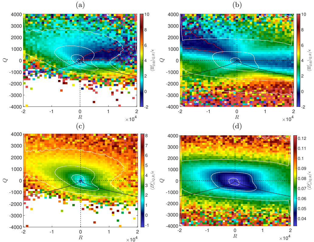
FIGURE 5. Conditional average of \Pi_{DR}^\ell and \mathcal{D}_v^\ell conditioned on the VGT second and third invariants Q and R . The white lines correspond to isovalues of the QR joint pdf. The red lines correspond to \langle \Pi_{DR}^\ell \rangle_{Q,R} = 0 . The black plain line corresponds to the Vieillefosse line 27R^2 + 4Q^3 = 0 . (a) Conditional average of \Pi_{DR}^\ell for \ell_c/\eta = 8 (case T4). (b) Conditional average of \Pi_{DR}^\ell for \ell_c/\eta = 150 (case T1). (c) Conditional average of \mathcal{D}_v^\ell for \ell_c/\eta = 8 (case T4). (d) Conditional average of \mathcal{D}_v^\ell for \ell_c/\eta = 150 (case T1).
