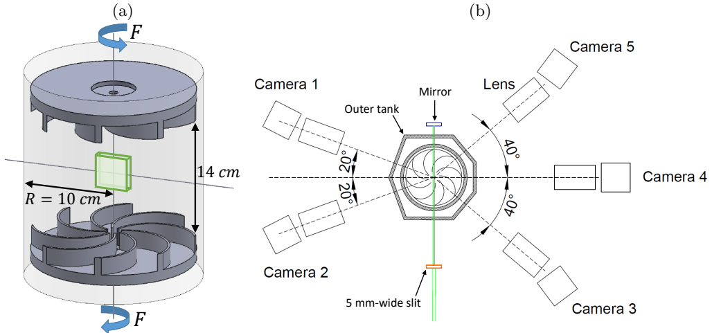
FIGURE 1. Experimental set-up. (a) Perspective view of the von Kármán flow geometry. The green area at the center is the measurement volume. (b) Top view of the whole set-up.
