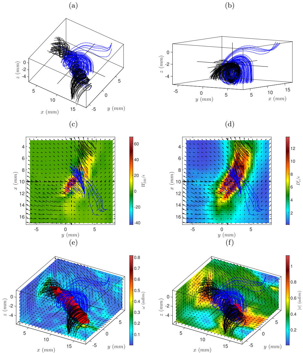
FIGURE 7. Velocity field around the 5 th extreme event of \Pi_{DR}^l of case T4. (a) Velocity streamlines. (b) Velocity streamlines from another point of view. (c) In-plane velocity field (arrows) and \Pi_{DR}^l field (color) in the (xy) plane containing the extreme event. (d) In-plane velocity field (arrows) and \mathcal{D}_v^l field (color) in the (xy) plane containing the extreme event. (e) In-plane velocity field (arrows) in three (xy) , (xz) and (yz) planes bounding the observed area, vorticity norm (color on these planes), velocity streamlines and isosurface of the vorticity norm (isolevel : 0.33). (f) In-plane velocity field (arrows) in three (xy) , (xz) and (yz) planes bounding the observed area, velocity norm (color on these planes), velocity streamlines and isosurface of the velocity norm (isolevel : 0.77). Blue streamlines are arriving at zones of large vorticity whereas black ones are leaving such zones.
