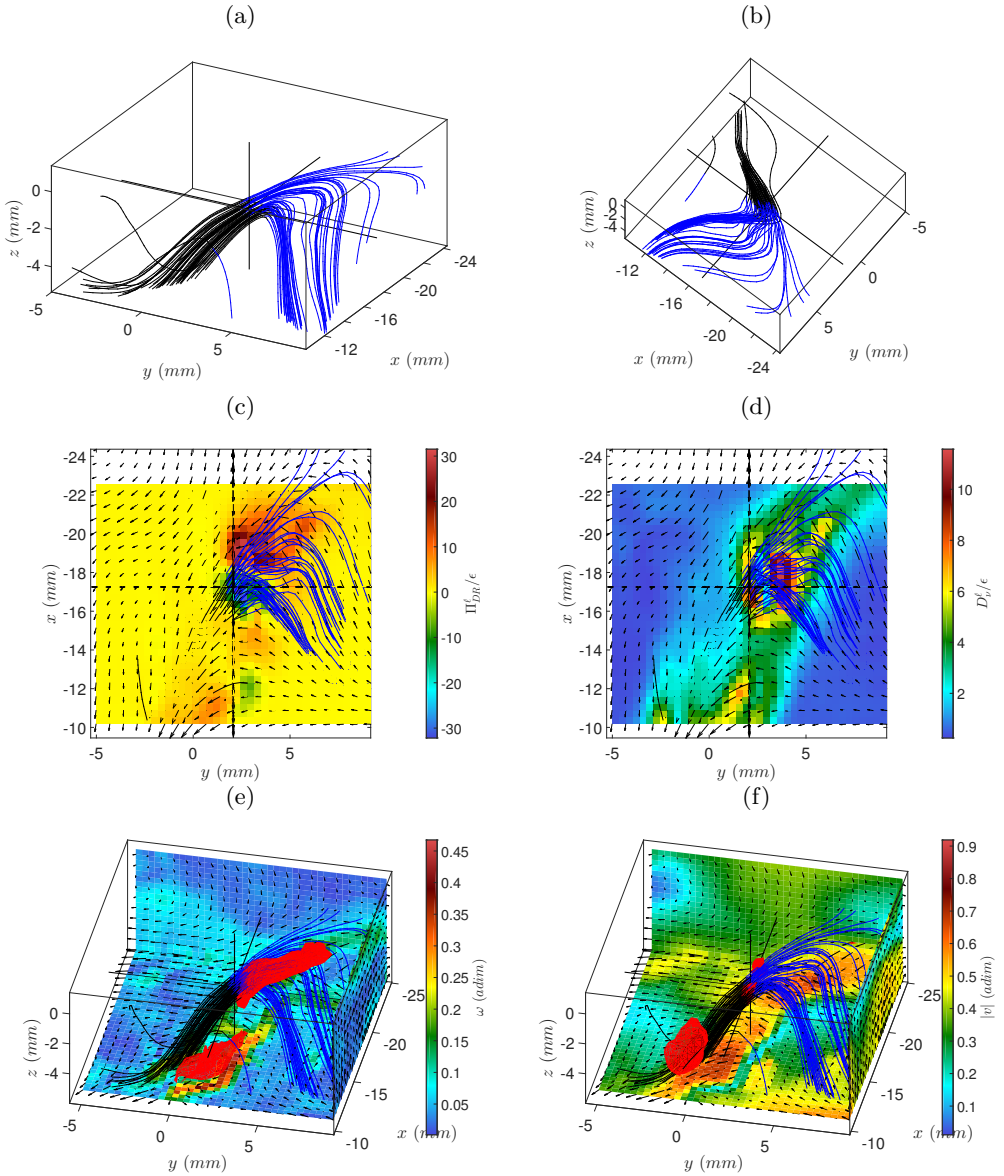
FIGURE 8. Velocity field around the 5 th negative extreme event of \Pi_{DR}^l of case T4. (a) Velocity streamlines. (b) Velocity streamlines from another point of view. (c) In-plane velocity field (arrows) and \Pi_{DR}^l field (color) in the (xy) plane containing the extreme event. (d) In-plane velocity field (arrows) and \mathcal{D}_v^l field (color) in the (xy) plane containing the extreme event. (e) In-plane velocity field (arrows) in three (xy), (xz) and (yz) planes bounding the observed area, vorticity norm (color on these planes), velocity streamlines and isosurface of the vorticity norm (isolevel : 0.33). (f) In-plane velocity field (arrows) in three (xy), (xz) and (yz) planes bounding the observed area, velocity norm (color on these planes), velocity streamlines and isosurface of the velocity norm (isolevel : 0.77). Blue streamlines are arriving around the extreme event of \Pi_{DR}^l whereas black ones are leaving the extreme zone.
