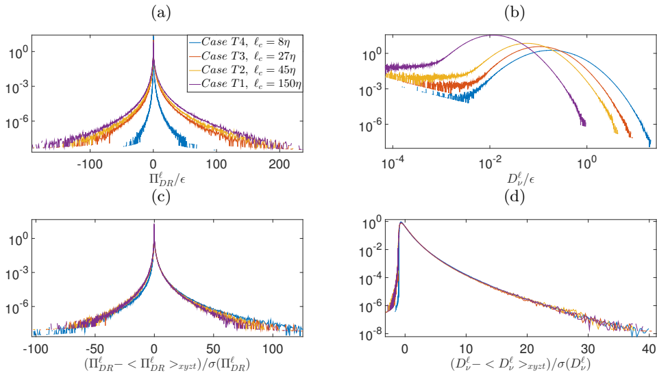
FIGURE 3. Probability density functions of \Pi_{DR}^\ell and of the viscous dissipation \mathcal{D}_\nu^\ell for cases T1 to T4. The vertical axes are in logarithmic coordinates and the horizontal axes in linear coordinates except for (b) where it is in logarithmic coordinates. Blue : \ell_c/\eta = 8 (case T4) ; red : \ell_c/\eta = 27 (case T3) ; orange : \ell_c/\eta = 45 (case T2) ; purple : \ell_c/\eta = 150 (case T1). (a) Pdf of \Pi_{DR}^\ell normalized by the global dissipation rate \epsilon (computed from torque measurements). (b) Pdf of \mathcal{D}_\nu^\ell normalized by the global dissipation rate \epsilon . (c) Centered-reduced pdf of \Pi_{DR}^\ell . (d) Centered-reduced pdf of \mathcal{D}_\nu^\ell .
