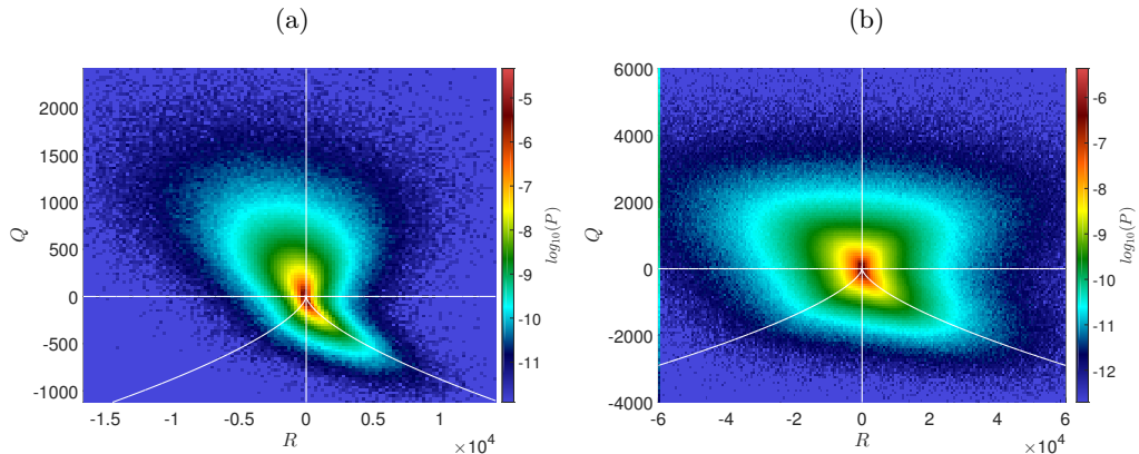
FIGURE 4. Joint pdfs of the second and third invariants of the VGT Q and R . (a) \ell_c/\eta = 8 (case T4). (b) \ell_c/\eta = 150 (case T1). White lines : Q = 0 , R = 0 and 27R^2 + 4Q^3 = 0 (Vieillefosse line).
