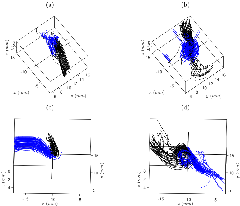
FIGURE 10. Impact of the frame of reference on the velocity field aspect. (a) Velocity streamlines around the 2^{nd} extreme event of \Pi_{DR}^{\ell} of case T4 seen in the laboratory frame of reference. (b) Velocity streamlines around the same event but in the frame of reference having a constant velocity (equal to the spatial average of the velocity over the observed field) with respect to the laboratory frame. (c) Velocity streamlines around the 2^{nd} negative extreme event of \Pi_{DR}^{\ell} of case T4 seen in the laboratory frame of reference. (d) Velocity streamlines around the same event but in the frame of reference having a constant velocity (equal to the velocity at the extreme point) with respect to the laboratory frame. Blue streamlines are arriving towards zones of high vorticity whereas black ones are leaving such zones. The three black lines intersect at the point where \Pi_{DR}^{\ell} is maximum.
