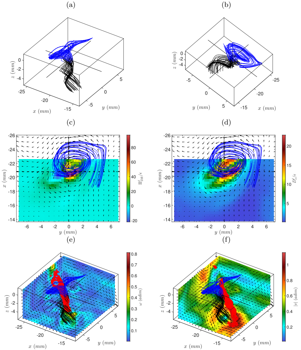
FIGURE 6. Velocity field around the 1 st extreme event of \Pi_{DR}^l of case T4. (a) Velocity streamlines. (b) Velocity streamlines from another point of view. (c) In-plane velocity field (arrows) and \Pi_{DR}^l field (color) in the (xy) plane containing the extreme event. (d) In-plane velocity field (arrows) and \mathcal{D}_v^l field (color) in the (xy) plane containing the extreme event. (e) In-plane velocity field (arrows) in three (xy) , (xz) and (yz) planes bounding the observed area, vorticity norm (color on these planes), velocity streamlines and isosurface of the vorticity norm (isolevel : 0.41). (f) In-plane velocity field (arrows) in three (xy) , (xz) and (yz) planes bounding the observed area, velocity norm (color on these planes), velocity streamlines and isosurface of the velocity norm (isolevel : 0.92). Blue streamlines are arriving around the extreme event of \Pi_{DR}^l whereas black ones are leaving the extreme zone.
