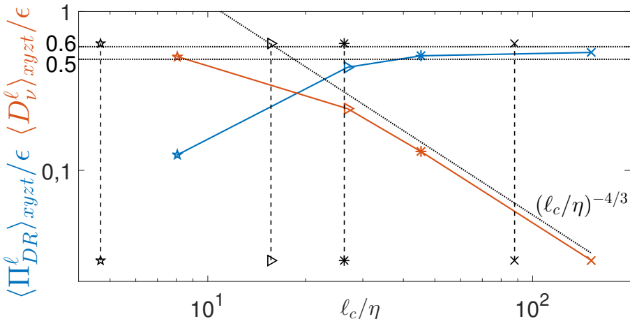
FIGURE 2. Space-time average of \Pi_{DR}^\ell (blue) and \mathcal{D}_\nu^\ell (red) with respect to scales. The vertical dashed lines correspond to the interrogation window size (divided by \eta ). Pentagons : \ell_c/\eta = 8 (obtained with case T4), triangles : \ell_c/\eta = 27 (obtained with case T3), star : \ell_c/\eta = 45 (obtained with case T2), cross : \ell_c/\eta = 150 (obtained with case T1). The dotted line corresponds to the scaling (\ell_c/\eta)^{-4/3} .
