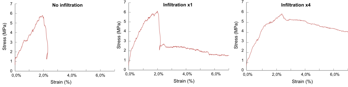
Figure 4: Stress-strain curves during mechanical testing (bending) of un-notched bars for the porous ceramic (left), and for the PCL/ceramic composites after 1 infiltration (middle) and 4 infiltration cycles (right). Infiltration with a 4% PCL solution. Note the displacement is measured by an LVDT sensor and not by the displacement of the fixture, explaining thus why the strain value may go backwards (center plot, around 2%). © (2020) J. Seuba et al. (10.6084/m9.figshare.15022263) CC BY 4.0 license https://creativecommons.org/licenses/by/4.0/ .
