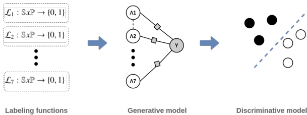
Figure 6: Data Programming pipeline for pairing
