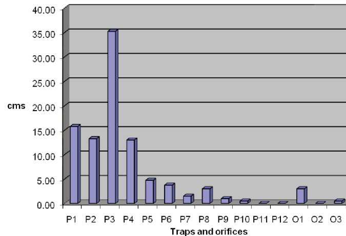
Figure 11: Thickness of sediment layer at sediment traps and in front of orifices – observed in July 2009
