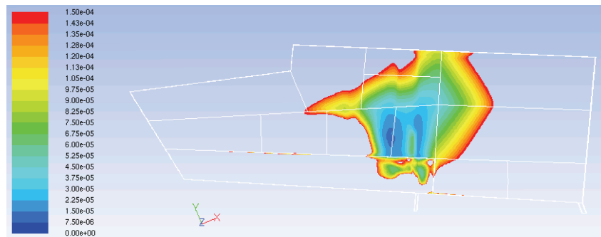
Figure 8: Areas corresponding to a turbulent kinetic energy < 0.00015 \text{ m}^2/\text{s}^2 - Q_{\text{inlet}} = 1 \text{ m}^3/\text{s}
