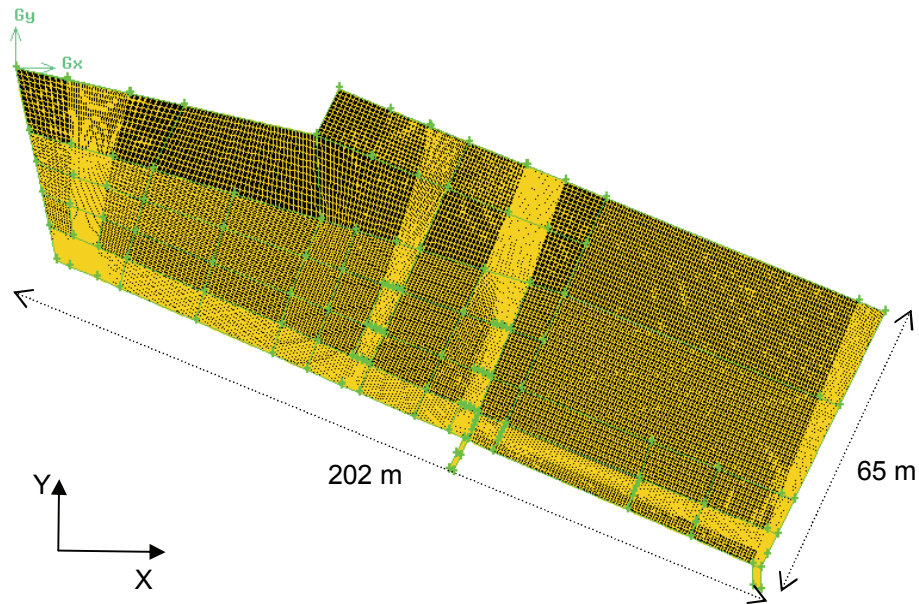
Figure 3: Computational hexahedral mesh of the basin for 3D simulations
