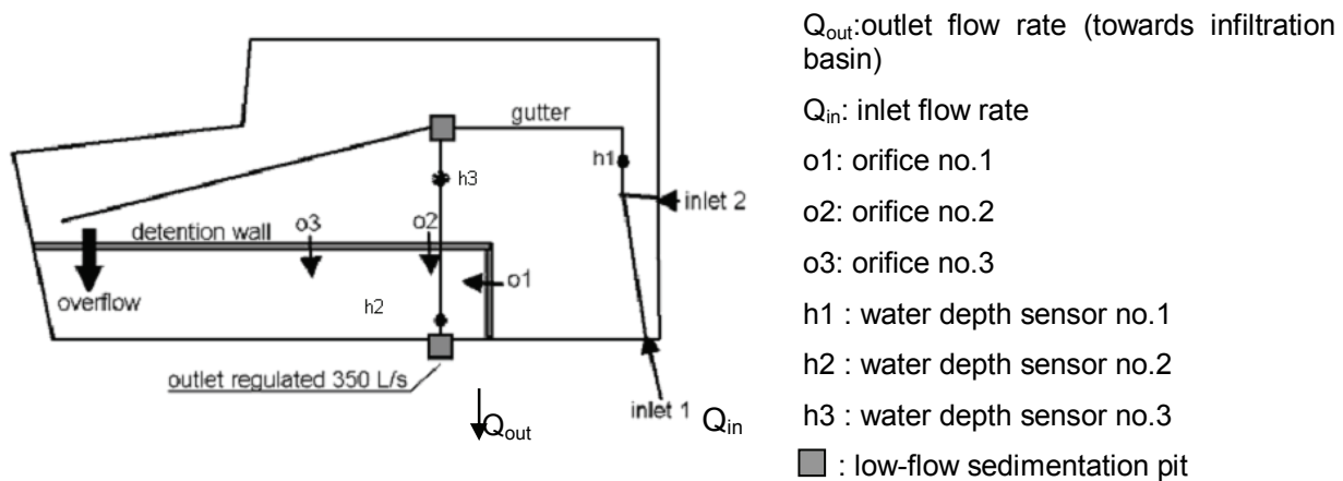
Figure 1: Scheme of the Django Reinhardt detention and settling basin after its retrofit in 2004 (Bardin and Barraud, 2004)
