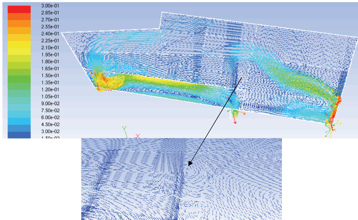
Figure 4: Free surface velocity field for the inlet flow rate of 0.3 \text{ m}^3/\text{s} and with the k-\epsilon turbulent model
