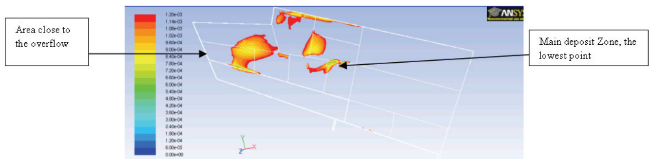
Figure 5: Areas corresponding to a friction coefficient < 0.0012 – Q_{\text{inlet}} = 1 \text{ m}^3/\text{s}
