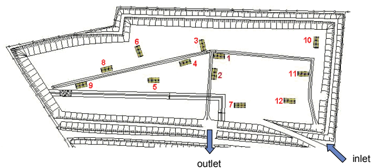
Figure 2: Sediment traps location and sampling devices (top view), (TORRES, 2008)
