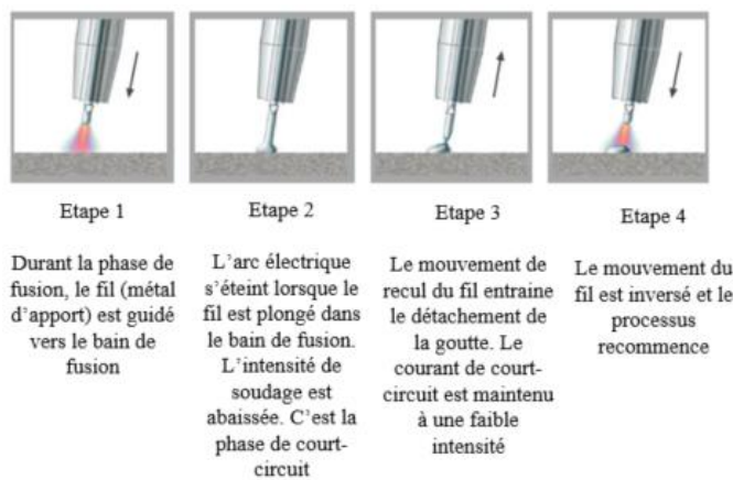
Figure 1. PRINCIPE DU CYCLE CMT
