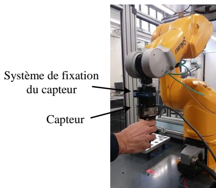
Figure 5. SYSTEME EXPERIMENTAL ROBOT STAUBLI TX2 60
