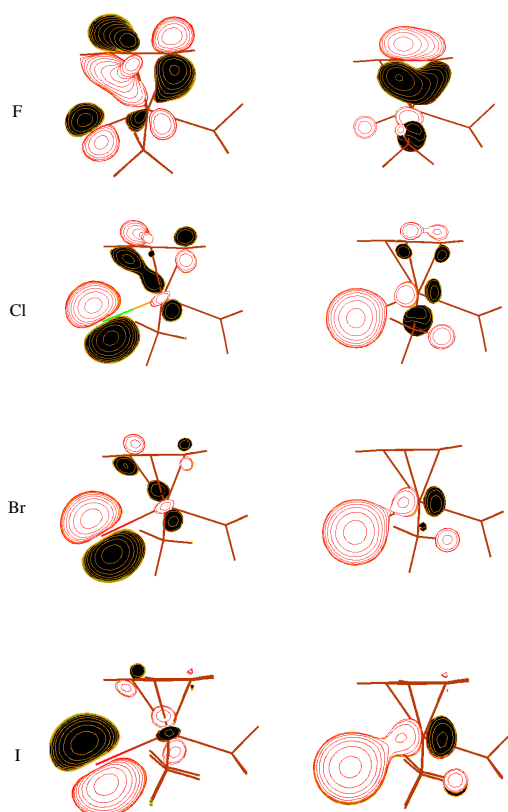
Figure 4. MOLDEN views of the 3rd (left) and 4th (right) highest MO for \text{CpMoX}(\text{PH}_3)_3 .
