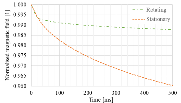
Fig. 3. Results for the simulated trapped field decay: (a) when the bulk experiences an oscillating AC field with a fixed stationary rotor (orange dashed line), (b) when the rotor is rotating at its synchronous speed (green dot-dashed line).
