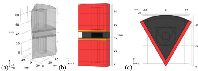
Fig. 2. (a) Geometry of the high-temperature bulk superconducting axial-gap synchronous machine finite-element model reduced to one sixth of the geometry by exploiting symmetry. (b) Side view with the A-formulation domain around the H-formulation domain hidden, (c) The top of the machine with the top vector and scalar potential domains removed for clarity, the vector potential to the right and left side of the H-formulation domain have the symmetric boundary conditions imposed. The A-formulation domains are shown in red, the magnetic scalar potential domains are yellow and the H-formulation domains are black.
