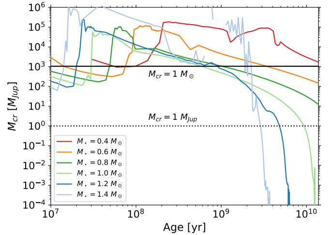
Fig. D.1. Evolution of the critical planetary mass M_{\text{cr}} as a function of the age of the system for stellar masses ( M_* ) between 0.4 and 1.4 M_\odot . Wave braking may occur for planetary masses higher than M_{\text{cr}} .
