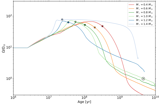
Fig. 7. Evolution of the surface rotation rate (scaled to the present Sun rotation rate) for stars with a mass ranging from 0.4 to 1.4 solar masses (Amard et al. 2019). The solar rotation rate at solar age is represented by a black circle. The colored squares correspond to the ZAMS in each model.
