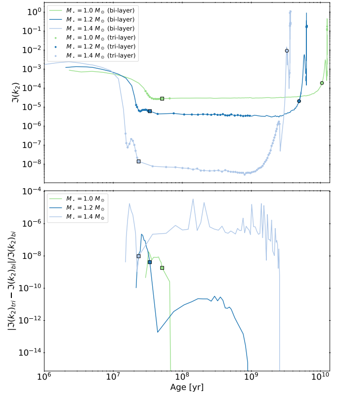
Fig. 12. Evolution of tidal dissipation in the case of a bilayer and a trilayer structure. Top: evolution of the tidal dissipation in the case of a bilayer (blue curves) and a trilayer (blue dots) structure as a function of time for stellar masses M_* = \{1 - 1.4\} M_\odot , with P_{\text{orb}} = 1 d. Bottom: time evolution of the relative difference of tidal dissipations derived from bilayer and trilayer structures. The colored squares correspond to the ZAMS in each model, and the colored circles show the TAMS.
