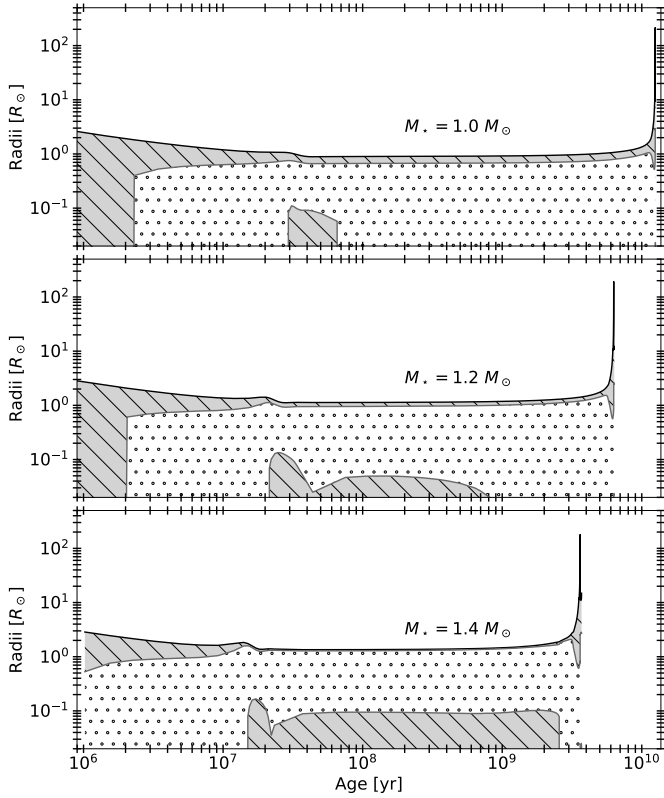
Fig. 11. Kippenhahn diagram showing the evolution of the internal structure of the nonrotating star for M_* = 1 M_\odot (top), M_* = 1.2 M_\odot (middle), and M_* = 1.4 M_\odot (bottom) from the PMS up to the end of the MS. The upper line represents the stellar radius in solar radii. The hatched gray areas depict convective regions, and the dotted areas stand for radiative regions.
