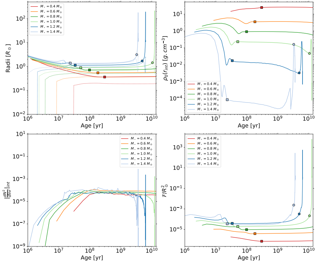
Fig. 4. Evolution of the stellar radius ( top left , plain line), the radius of the radiative zone ( top left , dotted line), the density at the interface core-envelope ( top right ), the gradient of the square of the Brunt–Väisälä frequency at the interface ( bottom left ) and the forcing term \mathcal{F} ( bottom right ) as a function of the age of the system for stellar masses ( M_* ) between 0.4 and 1.4 M_\odot , with P_{\text{orb}} = 1 d, a typical value for a hot Jupiter. The colored squares correspond to the ZAMS in each model, and the colored circles represent the TAMS.
