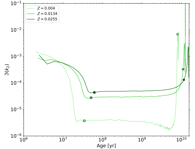
Fig. 10. Evolution of the tidal dissipation through gravity waves as a function of time for three different stellar metallicities, i.e., Z = 0.004 , Z = 0.0134 = Z_\odot , and Z = 0.0255 , with M_\star = 1 M_\odot and P_{\text{orb}} = 1 d. The colored squares correspond to the ZAMS in each model, and the colored circles show the TAMS.
