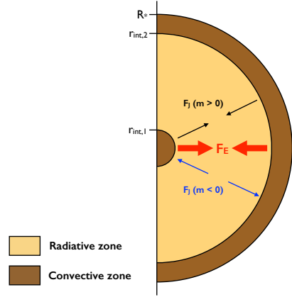
Fig. 3. Configurations of the radiative and convective spherical shells for the case of a trilayer structure. In brown we show the convective layer. In orange we plot the radiative layer. The red arrows represent the energy fluxes ( F_E ), the black arrows correspond to the angular momentum fluxes ( F_J ) for prograde waves ( m > 0 ), and the blue arrows stand for the angular momentum fluxes in the case of retrograde waves ( m < 0 ).
