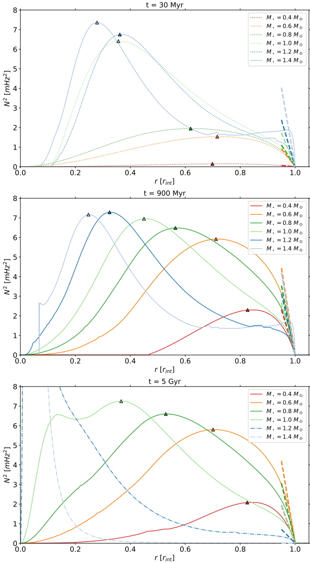
Fig. 5. Brunt–Väisälä frequency profiles as a function of the distance to the center of the star, normalized to the radius of its radiative zone, at 30 Myr ( top panel ), 900 Myr ( middle panel ), and 5 Gyr ( bottom panel ). The dotted profiles are situated in the PMS, the plain lines in the MS, and the dash-dotted lines in the post-MS phase. The colors correspond to the same stellar masses as in Fig. 4. The dashed lines correspond to the tangents to the N^2 profiles at the interface. The triangles indicate the position of the maximum Brunt–Väisälä frequency.
