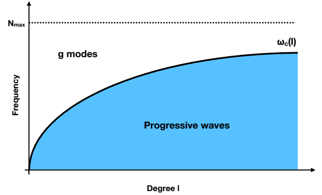
Fig. 2. Nature of internal gravity waves as a function of degree l and frequency. The dashed black line corresponds to the maximum value of the Brunt–Väisälä frequency N_{\text{max}} in the radiative zone. The black line corresponds to the cutoff frequency \omega_{\text{c}} as a function of the degree, marking the separation between standing g -modes (in white, above) and progressive internal gravity waves (in blue, below).
