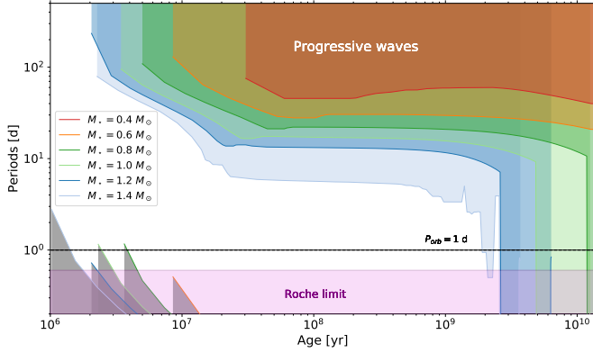
Fig. 8. Characteristic periods as a function of the age of the system for stellar masses between 0.4 and 1.4 M_{\odot} . In dark gray we plot the region corresponding to tidal frequencies greater than N_{\max} , for which no propagation of gravity waves is allowed. The colored areas correspond to orbital periods that are likely to excite progressive waves (with frequencies \omega < \omega_c ) for each stellar mass. In purple we show typical values corresponding to the Roche limit. The dashed black line corresponds to an orbital period of one day.
