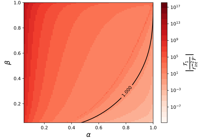
Fig. C.1. Value of \mathcal{T}_1/r_{\text{int}}^{-2}\mathcal{F} for all the possible values of \alpha = R_r/R_* and \beta = M_r/M_* . In black we show values of \alpha and \beta for which the ratio is equal to 1.
