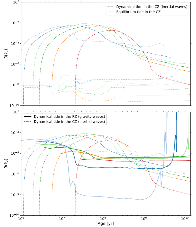
Fig. 9. Top: evolution of the dissipation of the dynamical tide through inertial waves (dashed lines) and of the equilibrium tide in the convective zone (dotted lines). Bottom: evolution of the dissipation of the dynamical tide through gravity waves (solid lines) and of the dynamical tide through inertial waves (dashed lines). Stellar mass ranges between 0.4 and 1.4 M_{\odot} . The colors correspond to the same masses as in Fig. 8.
