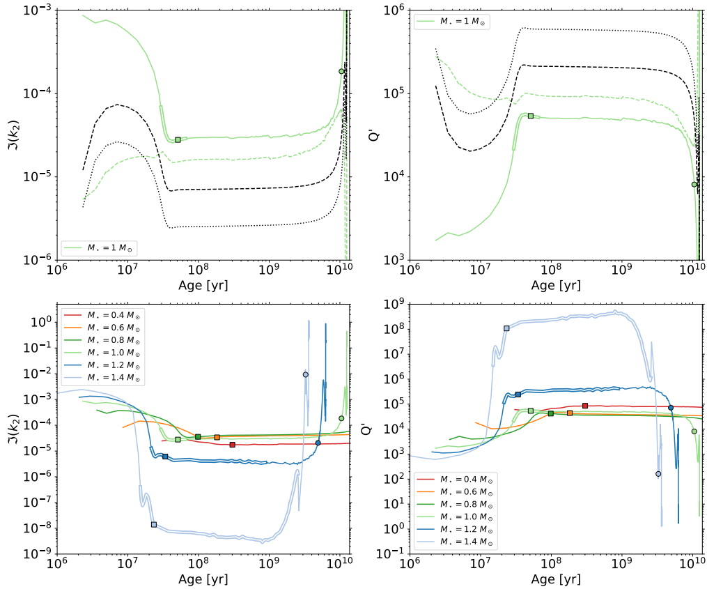
Fig. 6. Evolution of the tidal dissipation and the corresponding quality factor as a function of stellar mass and stellar age. Top left: evolution of the tidal dissipation as a function of time for M_{\star} = 1 M_{\odot} and P_{\text{orb}} = 1 d. Top right: time evolution of the corresponding tidal quality factor. In green we plot the prescription developed in our work. Dashed green shows the simplified prescription for a thin convective envelope. The dashed black line shows the Barker & Ogilvie (2010) prescription. The dotted black line represents the Goodman & Dickson (1998) prescription. Bottom left: evolution of the tidal dissipation as a function of time for stellar masses ( M_{\star} ) between 0.4 and 1.4 M_{\odot} , with P_{\text{orb}} = 1 d. Bottom right: time evolution of the corresponding tidal quality factor. The colored squares correspond to the ZAMS and the colored circles to the TAMS in each model. Double lines indicate the presence of a convective core. In this configuration, wave braking is unlikely to occur.
