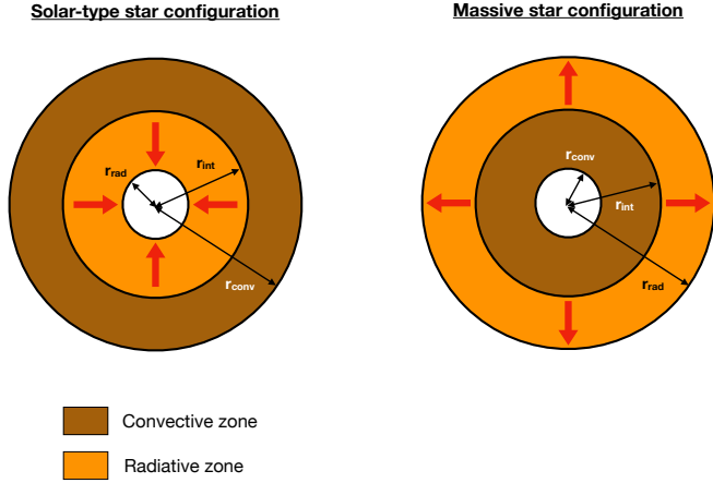
Fig. 1. Configurations of the radiative and convective spherical shells in our work. In brown we show the convective layer. In orange we plot the radiative layer. The red arrows represent the energy flux carried by tidal gravity waves.
