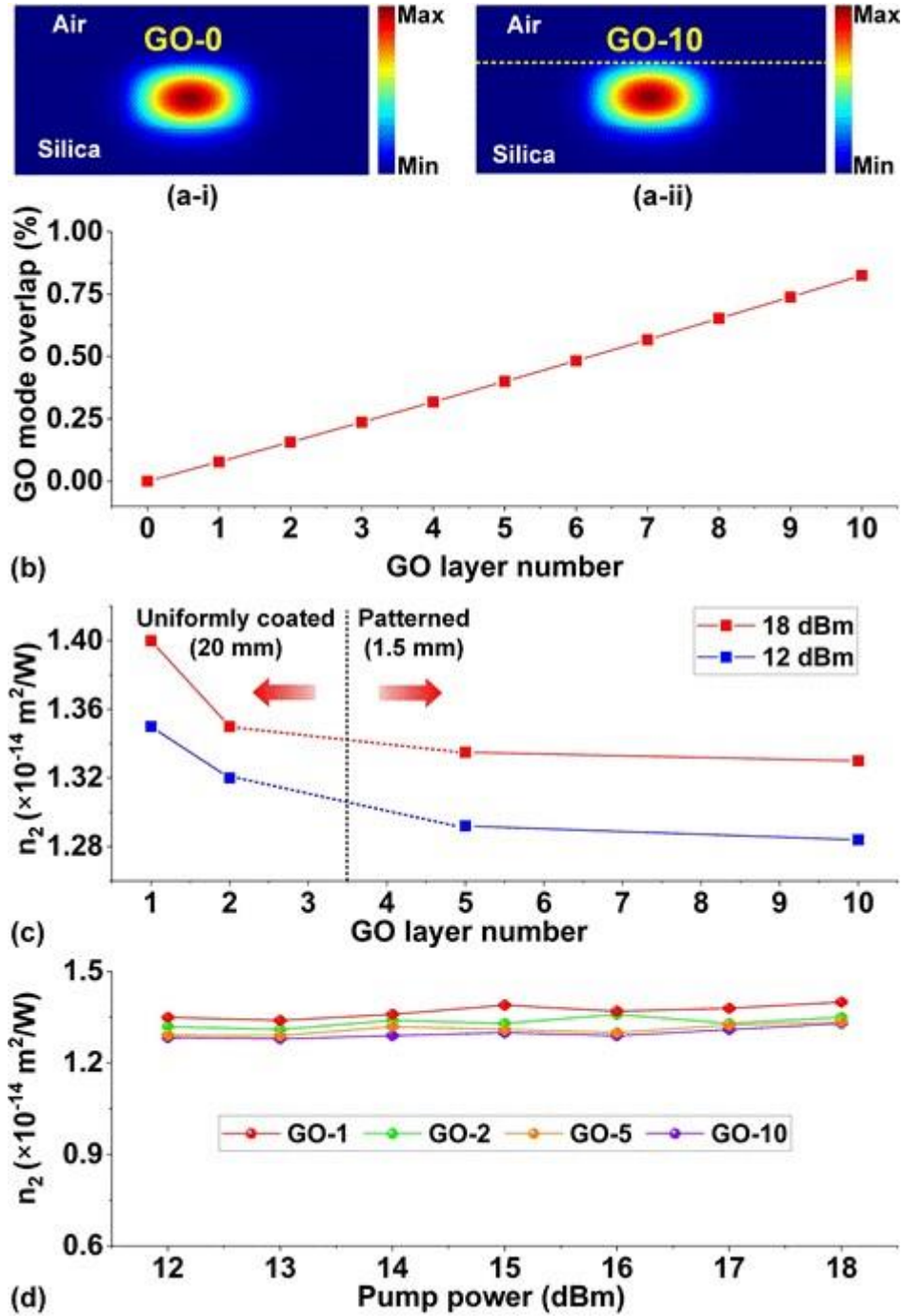
Figure 9. (a) TE mode profiles for the SiN waveguides (i) without GO and (ii) with 10 layers of GO. (b) Mode overlap with GO versus GO layer number for the hybrid waveguides. (c) n_2 of layered GO films versus GO layer number at fixed pump powers of 12 dBm and 18 dBm. (d) n_2 of layered GO films versus pump power for the hybrid waveguides with different numbers of GO layers.
