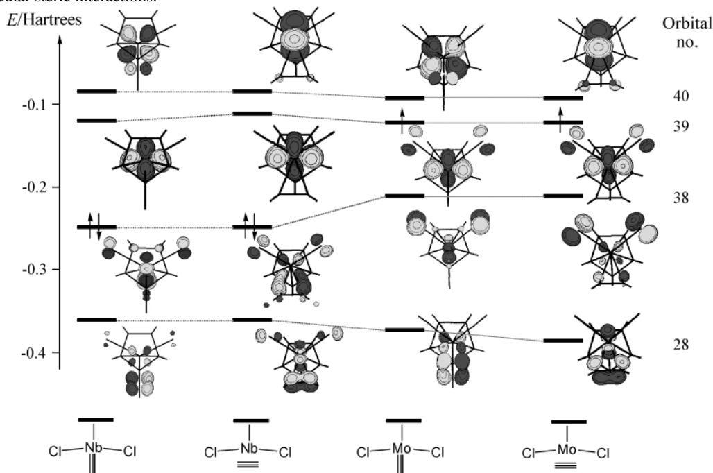
Fig. 3 Energy and shape of relevant orbitals for \text{CpMCl}_2(\text{HC}\equiv\text{CH}) ( M=\text{Nb}, \text{Mo} ).
