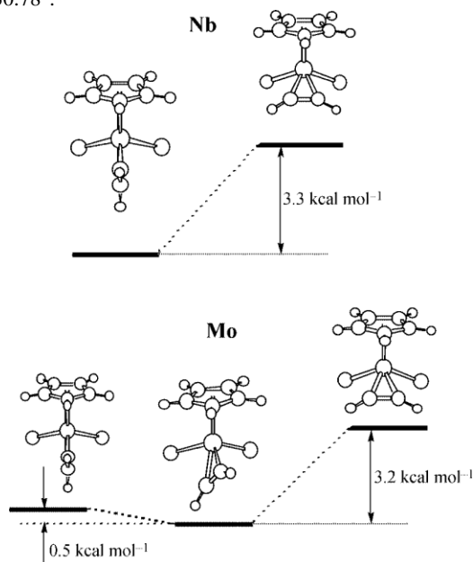
Fig. 2 B3LYP/LANL2DZ total energies for CpMCl 2 (HC≡CH) (M = Nb, Mo) at different ethyne conformations.
