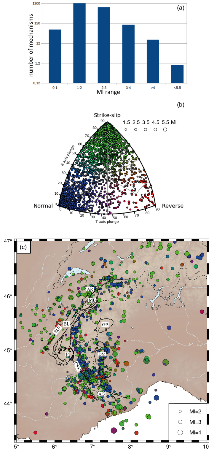
Figure 2. Set of the 2215 focal mechanisms computed in this study. (a) Histogram of magnitude distribution (local magnitude, M_1 ) for the computed focal mechanisms. (b) Kaverina diagram displaying the style of deformation of the mechanisms according to their T axis (tension axis) and B axis (null axis) plunges. Normal, reverse, and strike-slip deformation style corresponding to the vertical P , T , and B axes is indicated by circles in blue, red, and green, respectively. (c) Localization of the focal mechanisms colour-coded according to their classification in the Kaverina diagram in (b) . Note the different scale for events size between (b) and (c) . Black lines outline the crystalline massifs of the area. External crystalline massifs (Aiguilles Rouges, AR; Mont Blanc, MB; Belledonne, BL; Pelvoux, P; Argentera, AG) are separated from the internal crystalline massifs (Gran Paradiso, GP; Dora Maira, DM) by the Crustal Penninic Front (CPF). The Belledonne external massif is delineated by the Belledonne Fault (BLF) along its western flank.
