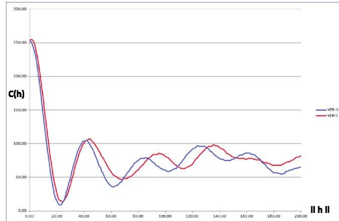
Figure 4: Example of covariograms for two different microstructures and associated cracking faces. C(\|h\|) represents the value of the covariogram and \|h\| is the norm of the translation vector
