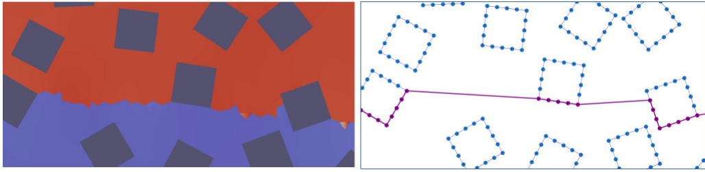
Figure 6: Discrete representation of a microstructure and crack path: on the right, the blue dots stand for the discretization points (y_i^E) and the purple path represents the XPER crack crossing the points (x_i^E) .
