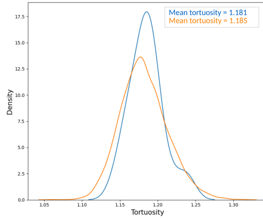
Figure 25: Comparison of the tortuosity densities constructed from the XPER simulations (blue) and the model predictions (orange) for microstructures with multiform aggregates (density obtained by kernel density estimate method)
