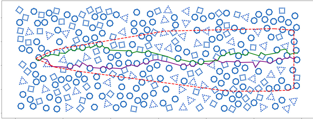
Figure 21: Example of path prediction for multiform aggregates: XPER simulation (purple), median path (green), region of confidence (dotted red curve)
