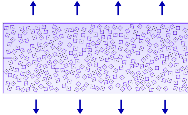
Figure 2: Test case submitted to traction (drawing process for the distribution of aggregates in the microstructure : HCPP (Hard Core Point Process))
