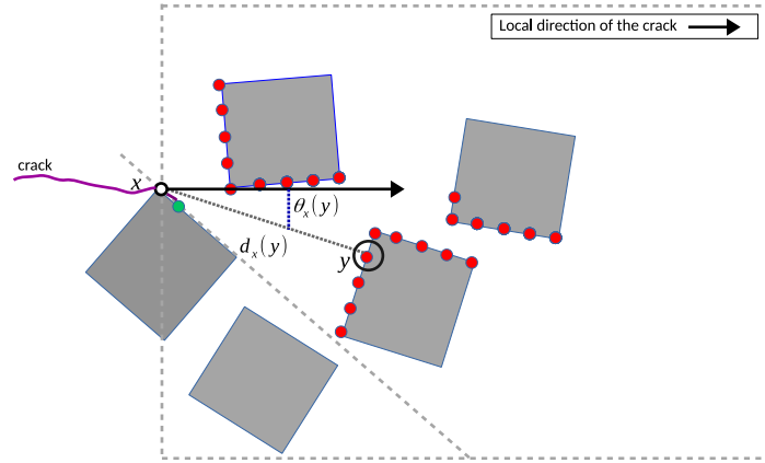
Figure 10: Illustration of the indicators of the candidate point y for the crack tip x in the configuration F1. The red points correspond to candidate points on neighbouring aggregates and the green point to the possibility of going along the same aggregate.
