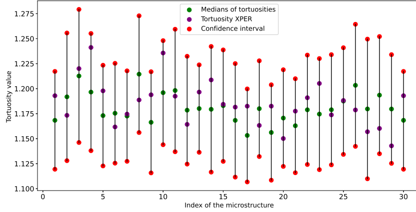
Figure 23: Tortuosity prediction on the test set (multiform aggregates): XPER simulations (purple), median predictions (green), uncertainty intervals (red)
