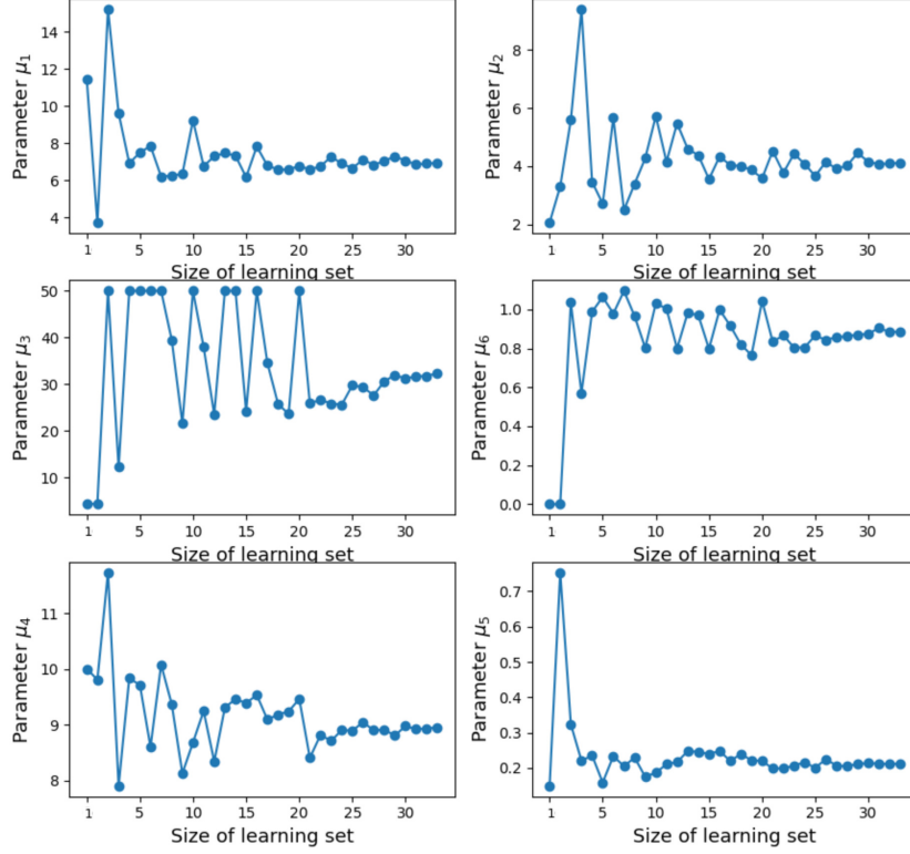
Figure 15: Parameter estimate with respect to the size of the training set in the F1 configuration. From top to bottom, parameters associated to \hat{\theta}_x (points on the same aggregate), to the interaction term (points requiring crossing the matrix) and to \hat{d}_x (points requiring crossing the matrix)
