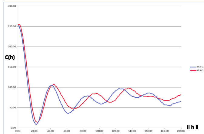
Figure 4: Example of covariograms for two different microstructures and associated cracking faces. C(\|h\|) represents the value of the covariogram and \|h\| is the norm of the translation vector
