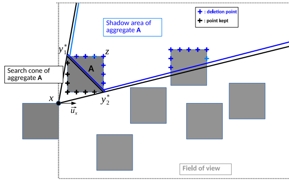
Figure 12: Illustration of Procedure 3.1 : construction of the shadow area (blue area) associated to aggregate A
