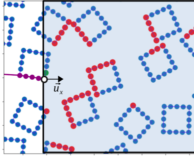
Figure 8: Field of view (F1): the green point stands for the candidate point belonging to the original aggregate, the red points stands for the candidate points on the other aggregates (implying to cross the matrix). The purple line stands for the path of the crack
