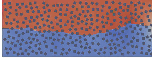
Figure 3: Crack path (colour discontinuity) obtained with XPER for the case described in the Figure 2. The colours stand for the vertical displacement.
