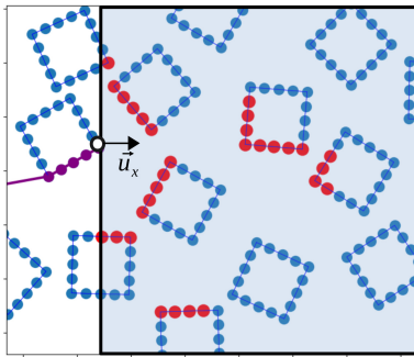
Figure 9: Field of view (F2) : the red points represent the candidate points on the other aggregates (implying to cross the matrix). The purple line stands for the path of the crack.
