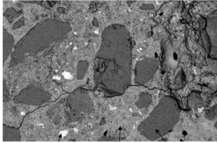
Figure 1: Example of a crack that propagates and follows the aggregate-matrix interface
