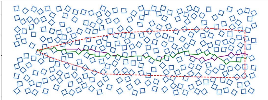
Figure 17: Example of path prediction for square aggregates: XPER simulation (purple), median path (green), region of confidence (dotted red curve)
