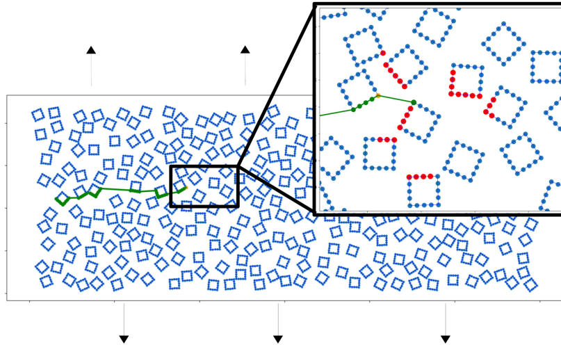
Figure 14: Illustration of the prediction (procedure 3.1) in the F2 configuration with a zoom on the region of interest. The field of view is orientated with respect to a propagation direction orthogonal to the stress effort. The orange point is the crack tip, the red points are candidate points in the field of view where the probability to be reached is evaluated, the green points are the candidate points selected by the model
