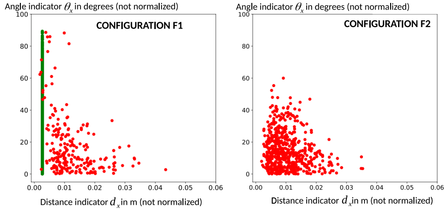
Figure 13: Indicator values in configurations F1 and F2 associated to points on the crack for 35 microstructures with square aggregates. Each point represents a couple of not normalized values (d_x, \theta_x) . The red dots stand for candidate points present on neighbouring aggregates (cross the matrix) and the green dots stand for the candidate points belonging to the same aggregate
