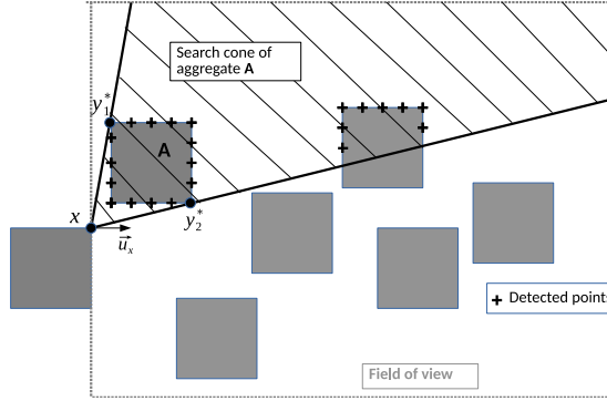
Figure 11: Illustration of Procedure 3.1 : construction of the search cone (hatched area) associated to aggregate A.
