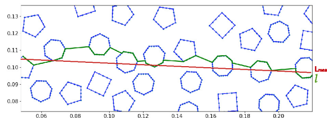
Figure 5: Representation of the tortuosity : \tau = \frac{l}{L_{mean}}
