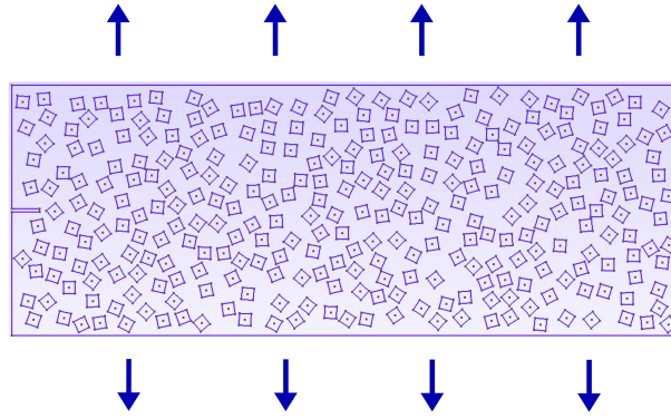
Figure 2: Test case submitted to traction (drawing process for the distribution of aggregates in the microstructure : HCPP (Hard Core Point Process))
