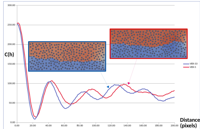
Figure 4: Comparison of two covariograms for two different microstructures
