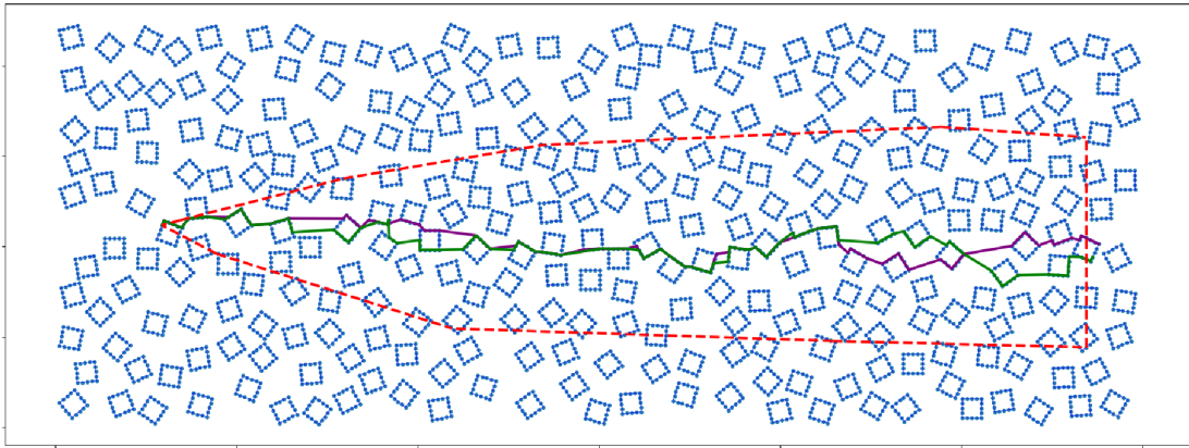
Figure 17: Example of path prediction for square aggregates: XPER simulation (purple), median path (green), region of confidence (dotted red curve)
