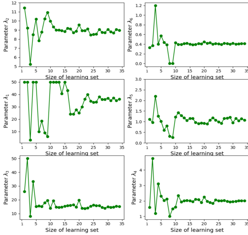
Figure 16: Parameter estimate with respect to the size of the training set in the F2 configuration. From top to bottom, parameters associated to \vec{d}_x , to the interaction term and to \vec{\theta}_x
