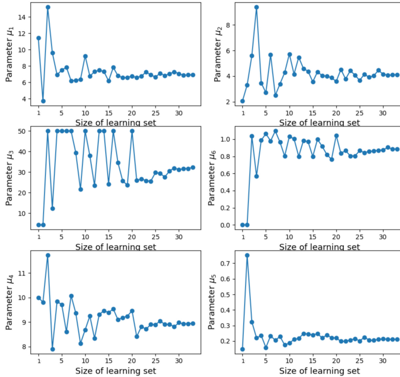
Figure 15: Parameter estimate with respect to the size of the training set in the F1 configuration. From top to bottom, parameters associated to \theta_x (points on the same aggregate), to the interaction term (points requiring crossing the matrix) and to \tilde{d}_x (points requiring crossing the matrix)
