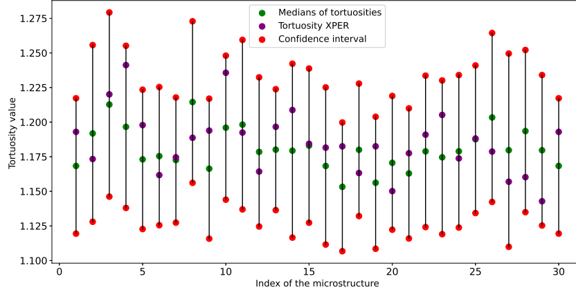
Figure 23: Tortuosity prediction on the test set (multiform aggregates): XPER simulations (purple), median predictions (green), uncertainty intervals (red)
