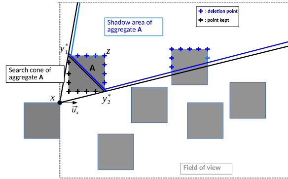
Figure 12: Illustration of Procedure 3.1 : construction of the shadow area (blue area) associated to aggregate A
