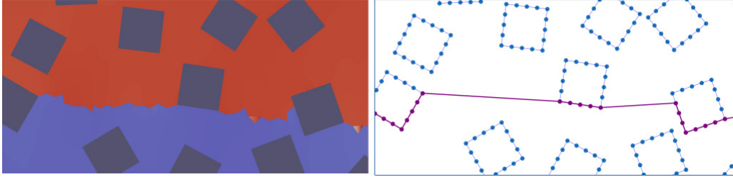
Figure 6: Discrete representation of a microstructure and crack path: on the right, the blue dots stand for the discretization points ( y_i^E ) and the purple path represents the XPER crack crossing the points ( x_i^E ).
