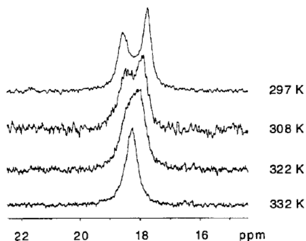
Figure 5. ^{31}\text{P}\{^1\text{H}\} NMR spectra at variable temperature for complex 8 in \text{CD}_3\text{CN} .
