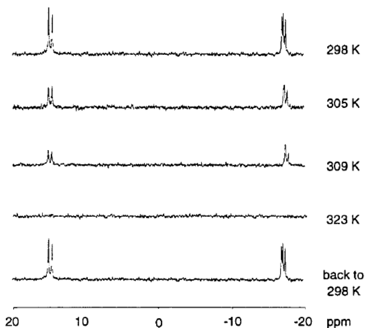
Figure 4. ^{31}\text{P}\{^1\text{H}\} NMR spectra at variable temperature for phosphine exchange on complexes 7a , 7b , and 7c in \text{CD}_3\text{CN} .
