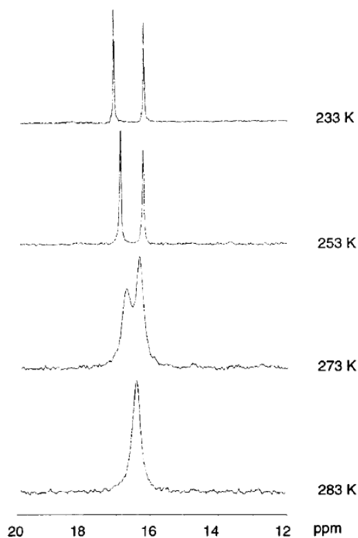
Figure 2. ^{31}\text{P}\{^1\text{H}\} NMR spectra at variable temperature for complex 4 in \text{CDCl}_3 .
