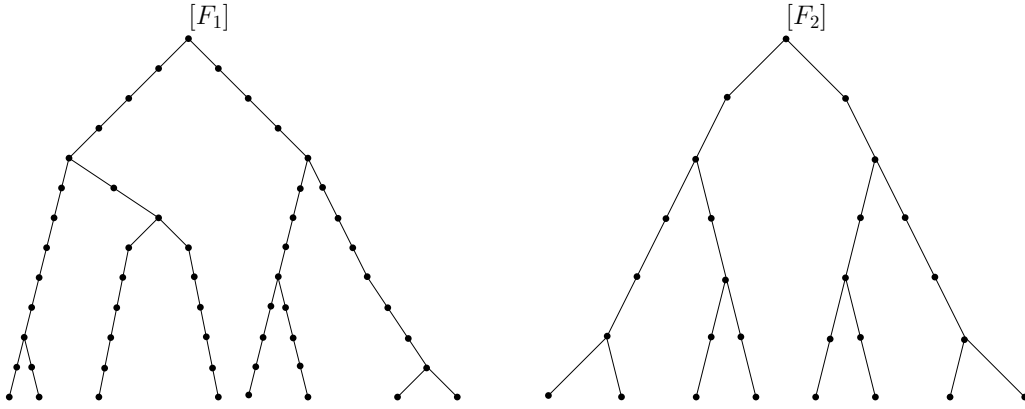
Figure 4: Two fig trees of scale n = 2 but with different heights.
