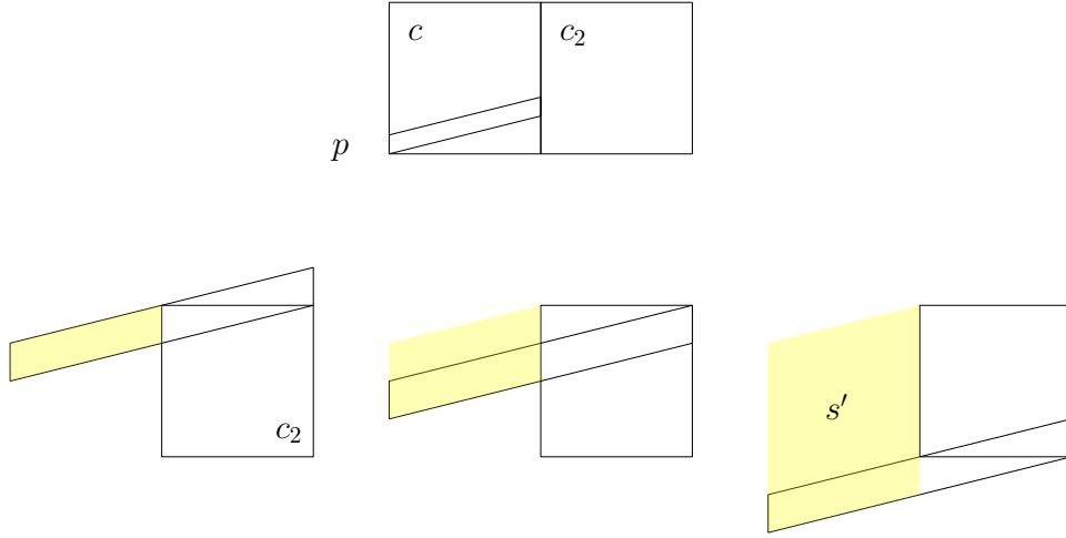
Figure 10: An illustration of the situation in proposition 9. We have s' \subset \{M_p \mathbb{1}_{c_2} > \frac{1}{4}\} and s' \subset h(c) . Moreover |s'| is quite large i.e. we have |s'| \simeq |c| .
