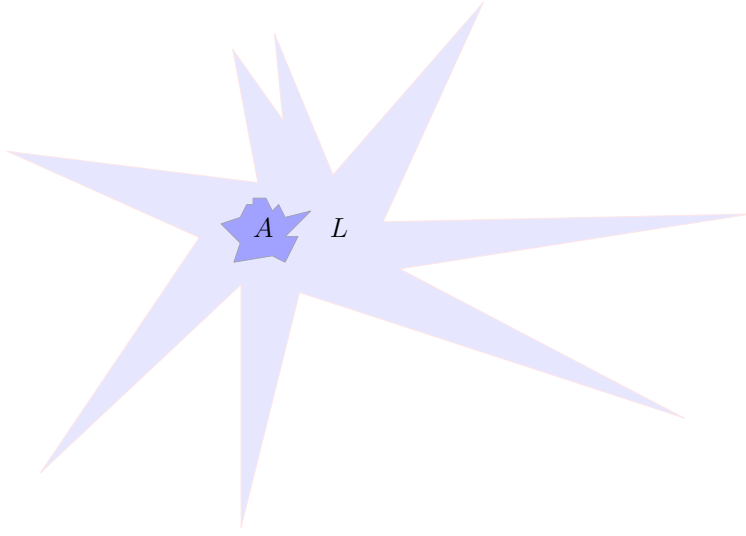
Figure 1: Suppose that for any \epsilon > 0 one can find a set A such that the set L := \{M_G \mathbb{1}_A > \frac{1}{2}\} is much bigger than A i.e. |A| \ll |L| . In this case, M_G is a bad operator.
