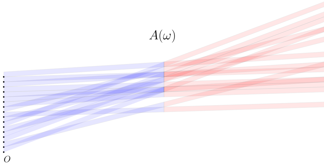
Figure 7: A realisation of A(\omega) . Even if this is not flagrant here, the point is that the blue area tends to become \log(n) times bigger than the red area.
