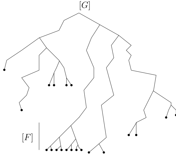
Figure 5: We can compute on this example the analytic split of G ; we have \lambda_{[G]} = 3 .
