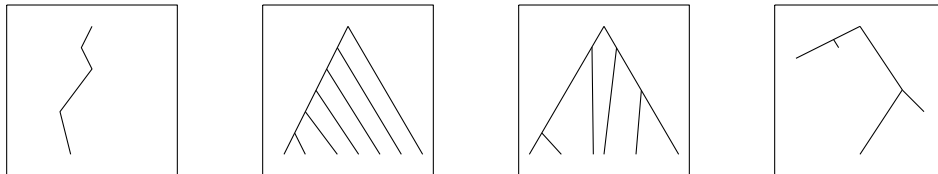
Figure 8: The first three trees are infinite and have no leaf : one can compute their split, it is respectively s_{[T]} = \lambda_{[T]} = 0, 1, 3 . The last tree is not infinite and do have leaves. However we have \lambda_{[T]} = 1 .
