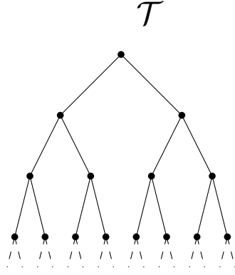
Figure 3: The family T composed of pulled-out parallelograms. We develop a language adapted to its structure of binary tree.
