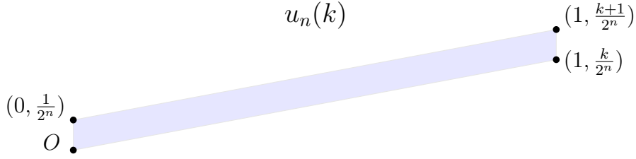
Figure 2: A parallelogram of scale n .
