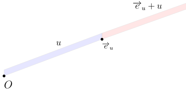
Figure 6: A representation of d(u) .
