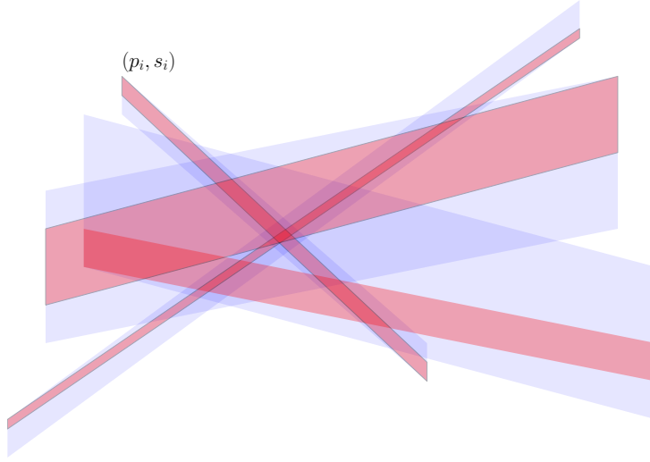
Figure 9: Each red parallelogram s_i satisfy s_i \subset p_i and |s_i| \geq \frac{1}{4}|p_i| where p_i is a blue parallelogram. Hence, the red shaded area takes at least \simeq \frac{1}{4} of the blue one.
