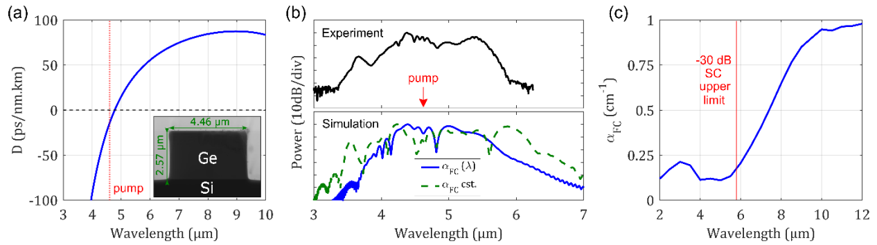
Fig. 1. (a) Dispersion parameter of the germanium on silicon waveguide with a 4.46 \mu\text{m} \times 2.57 \mu\text{m} cross-section. A Scanning Electron Microscope image of the waveguide is shown in the inset. (b) Top: output experimental supercontinuum for 22 mW (3.3 kW) coupled average (peak) power. Bottom: simulated supercontinuum considering wavelength dependent (continuous blue line) and constant (dashed green line) free-carrier absorption. (c) Free-carrier absorption coefficient as a function of wavelength at 1 cm length along the waveguide.
