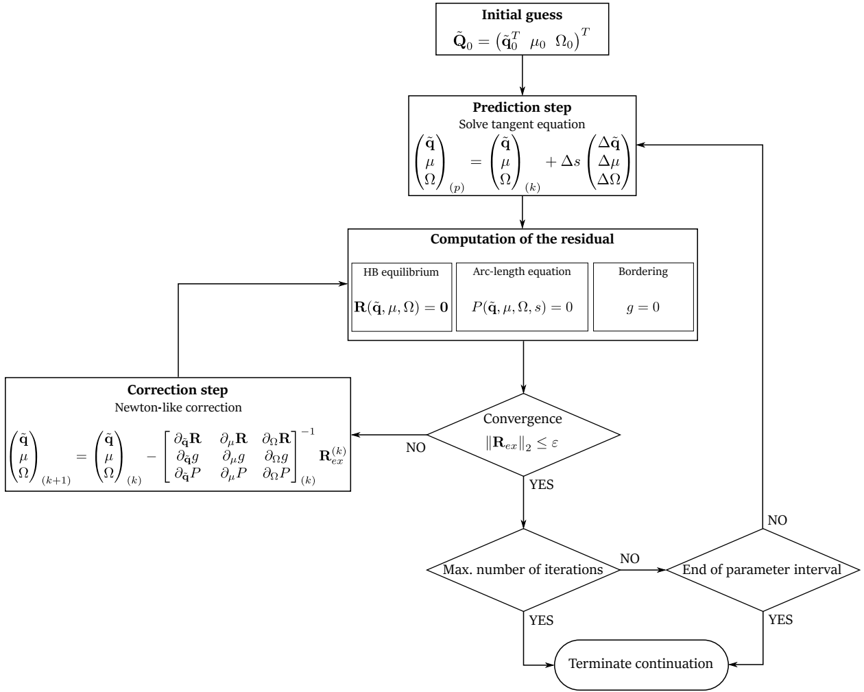
Fig. 4: Flow chart of the bifurcation tracking algorithm
