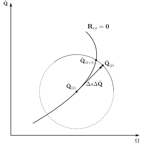
Fig. 2: Illustration of the arc-length continuation.
