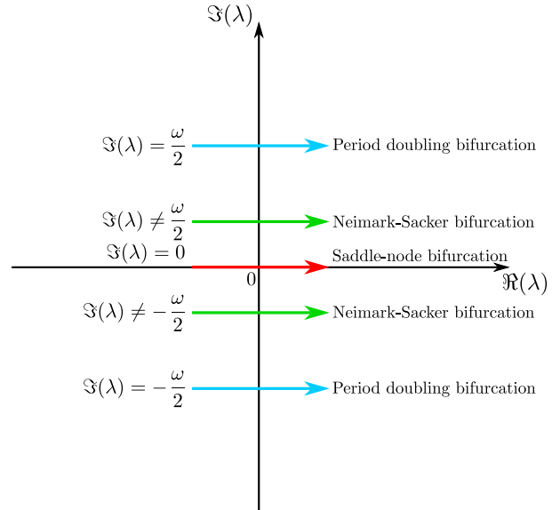
Fig. 3: Bifurcation scenarii depending on the Imaginary part of the crossing eigenvalue.
