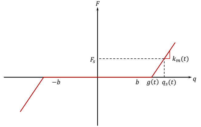
Fig. 6: Nonlinear force model.
