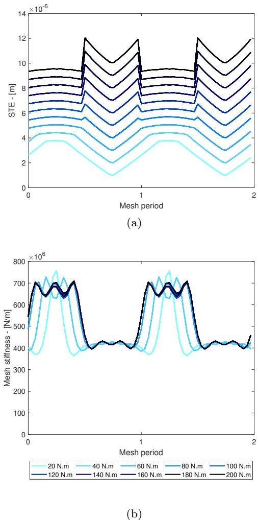
Fig. 7: Time evolution of the static transmission error and mesh stiffness computed by solving Eq. (38) and reconstructed with 6 harmonics for torque values ranging from 20 N·m (—) to 200 N·m (—)
