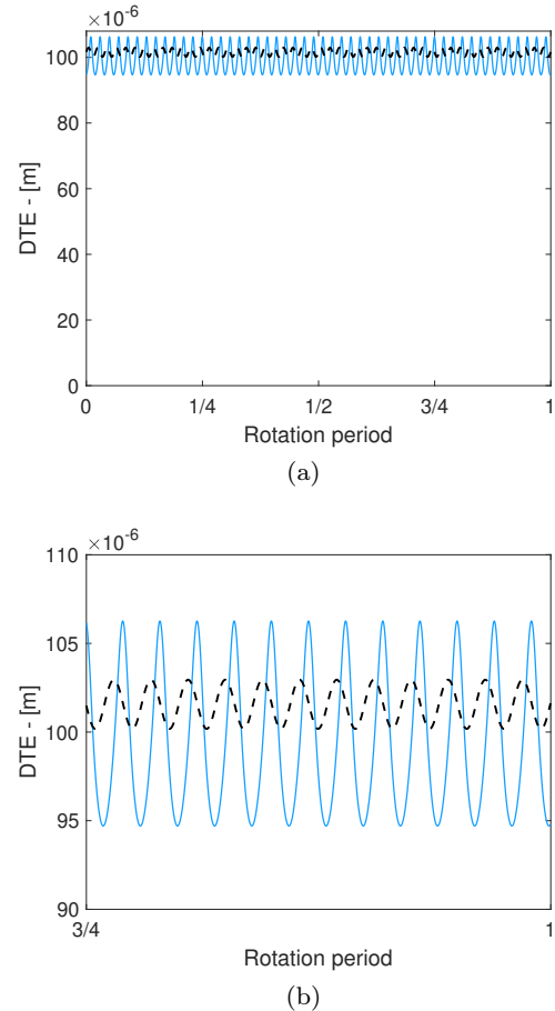
Fig. 10: Dynamic transmission error on top of the primary resonance after the saddle-node bifurcation (a) and close-up (b). The DTE and the gap limit are plotted as a blue solid line (—) and black dashed line (---), respectively.
