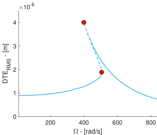
Fig. 9: Forced response of the gear model for an input torque T = 20 N·m.
