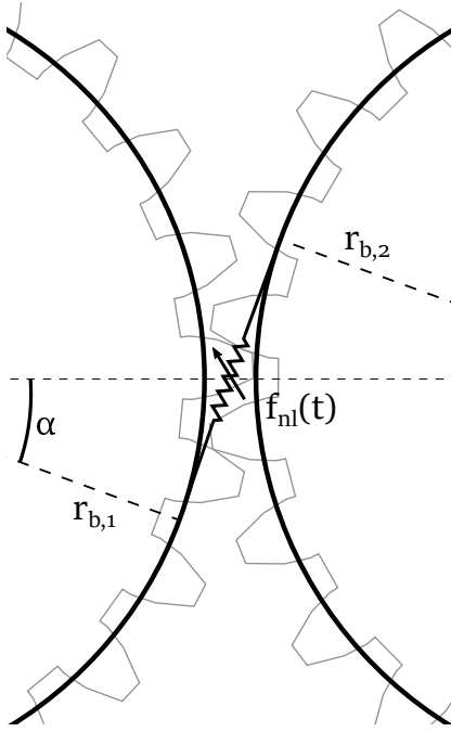
Fig. 5: Nonlinear gear model.
