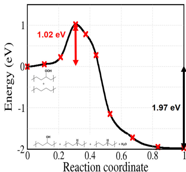
Figure 9. Calculated energy profile for reaction 6 of Figure 2 in a model of crystalline PE. The calculated outcome is here different from the commonly accepted one, giving instead two alkyl radicals and an alcohol, plus a water molecule.
