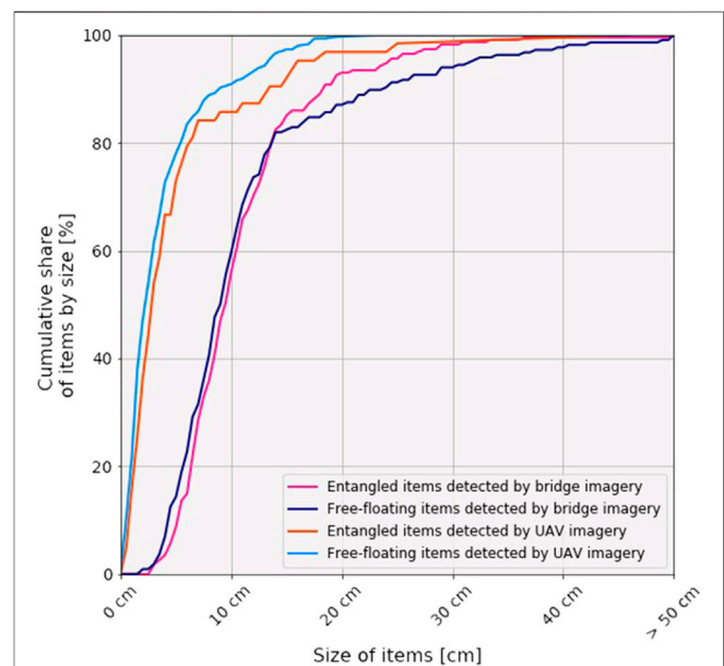
FIGURE 7 | Size distribution of plastic items from the bridge ( n = 444 ) and UAV imagery ( n = 359 ).
