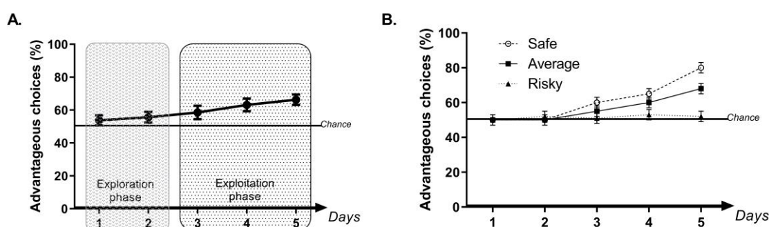
Figure 5. Example of the results usually obtained while doing the Mouse Gambling Task.
