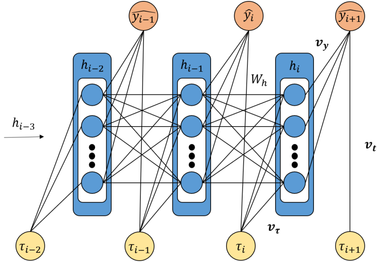
Figure 2: A recurrent neural network.
