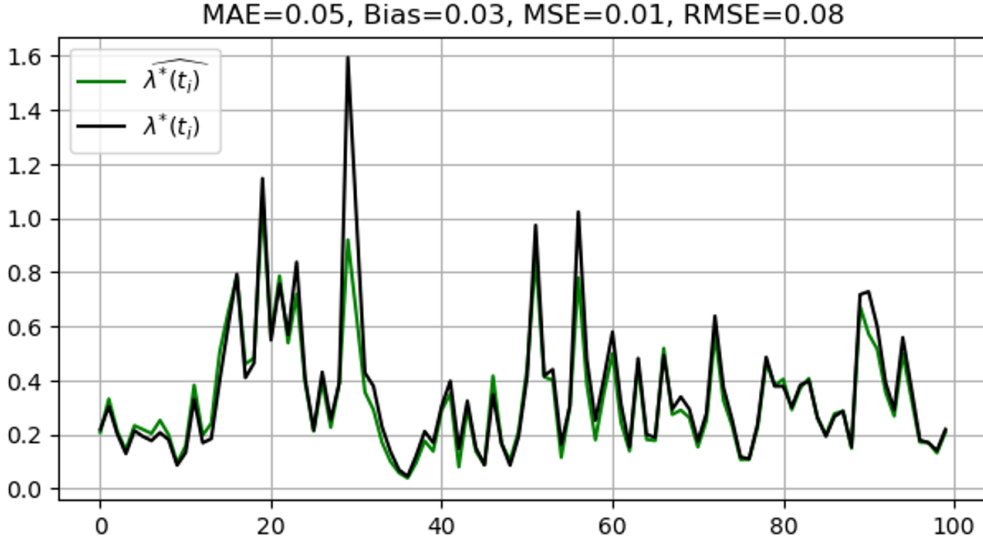
Figure 6: Neural network estimation of intensity function (green) against intensity function of self-correcting process generating artificial data (black).
