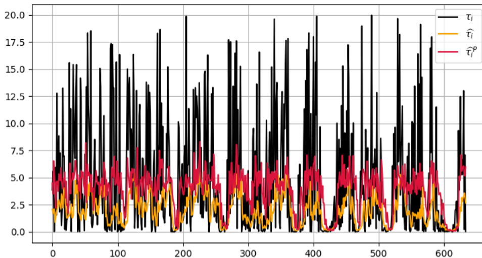
Figure 9: Next arrival prediction on the testing set. The neural network estimation is in yellow and the standard parametric estimation is in salmon. Actual next arrival time is in black.
