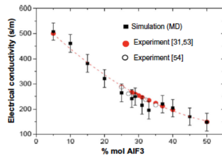
Fig. 6—Electrical conductivity of NaF-AlF 3 molten baths at 1032 °C between MD and experiments [50,52,53]
