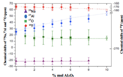
Fig. 15—NMR chemical shifts in the liquid of nuclei ^{27}\text{Al} , ^{17}\text{O} , ^{23}\text{Na} in the main axis, and ^{19}\text{F} in the secondary axis. Experimental values in markers empty and values calculated in full markers for the [\text{NaF}-\text{AlF}_3]_{\text{CR}2,2}-\text{Al}_2\text{O}_3 system.
