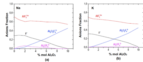
Fig. 10—Anion fractions deduced from the chemical shifts of the NMR at HT for molten \text{MF-AlF}_3\text{-Al}_2\text{O}_3 systems (a) \text{M} = \text{Na} on the left (b) \text{M} = \text{K} on the right) for a cryolite ratio 2.2.
