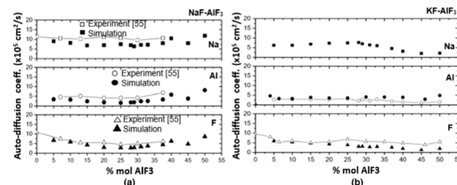
Fig. 8—Auto-diffusion coefficients of alkali ions, aluminum, and fluorine ions in (a) -NaF-AlF 3 and (b) -KF-AlF 3 at 1032 °C as a function of mol pct of AlF 3 from MD simulation and experimental data. [49]
