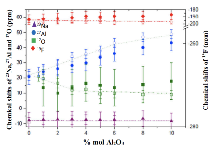
Fig. 13—NMR chemical shifts in the liquid of ^{27}\text{Al} , ^{17}\text{O} , ^{23}\text{Na} nuclei in the main axis and ^{19}\text{F} in the secondary axis. Experimental values in markers empty, and values were calculated in full markers for the [\text{NaF}-\text{AlF}_3]_{\text{CR}2,2}-\text{Al}_2\text{O}_3 system.
