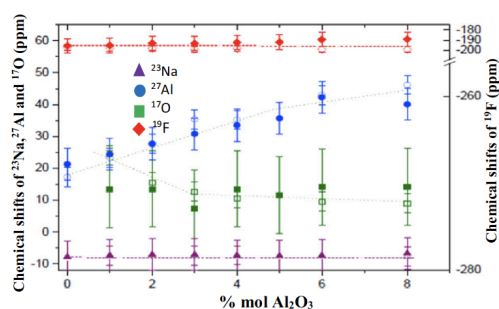
Fig. 14—NMR chemical shifts in the liquid of nuclei ^{27}\text{Al} , ^{17}\text{O} , ^{23}\text{Na} in the main axis, and ^{19}\text{F} in the secondary axis. Experimental values in empty markers and values calculated in full markers for the [\text{NaF}-\text{AlF}_3]_{\text{CR}3}-\text{Al}_2\text{O}_3 system.
