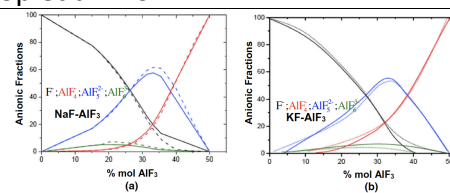
Fig. 4—Anionic fractions of the different species present in (a)-NaF-AlF 3 baths and (b)-KF-AlF 3 . In solid lines, the data are from the NMR experiments. Dotted data are from Raman experiments. [49]
