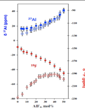
Fig. 3—Chemical shifts at constant superheat of 20 °C between 0 to 50 mol pct of \text{AlF}_3 in NaF-AlF 3 system (open symbols) and KF-AlF 3 (full markers).
