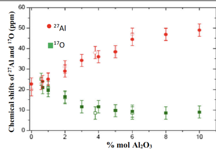
Fig. 9—Chemical shifts at high temperature for the ^{27}\text{Al} and ^{17}\text{O} nuclei of the system \text{NaF-AlF}_3\text{-Al}_2\text{O}_3 with a cryolite ratio 2.2 (full markers) and cryolite ratio 3 (empty markers).
