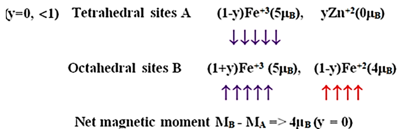
Figure 2. The spin magnetic moment per formula unit of Zn_yFe_{3-y}O_4 for y = 0 and 1.
