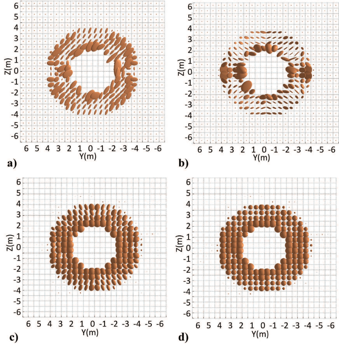
Fig. 8. Frontal views of the 3D upscaled coefficients, from left to right and up to down, N_{ij} , S_{ij} , B_{ij}^{(0)} (ellipsoids) and 1/M^{(0)} (spheres) in the first transverse layer ( Y, Z ) with X \in [10.0 \text{ m}, 9.5 \text{ m}] .
