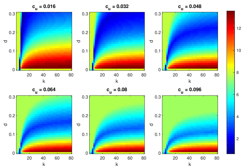
Figure 10: Time t_c (s) to reach 50% of the initial amplitude as a function of parameters k , d and c_u .
