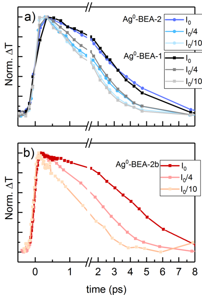
Figure 6. Kinetics of the transmission change probed at \lambda_{\text{probe}} = 380 nm, with different pump intensity ( \lambda_{\text{pump}} = 400 nm), a) I_0 = 1.2 mJ/cm 2 , Ag 0 -BEA-1 and Ag 0 -BEA-2, and b) I_0 = 1.2 mJ/cm 2 , Ag 0 -BEA-2b.
